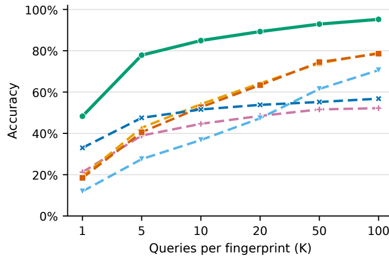
Ministral-3-8B-Instruct-2512
