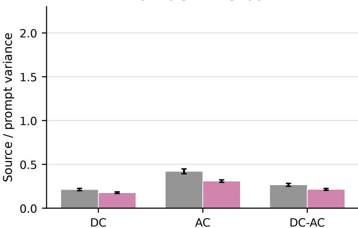
OLMo-3-7B-Instruct
