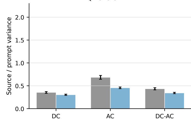
Qwen3.5-27B
