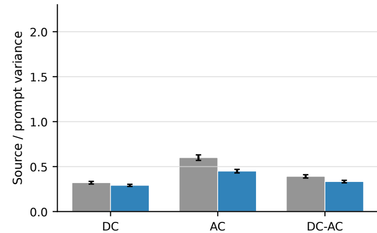
Qwen3.5-27B
