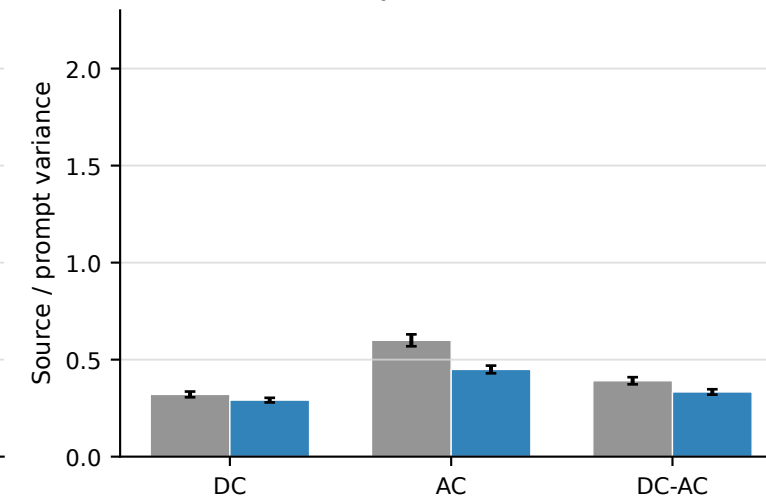
Qwen3.5-9B
