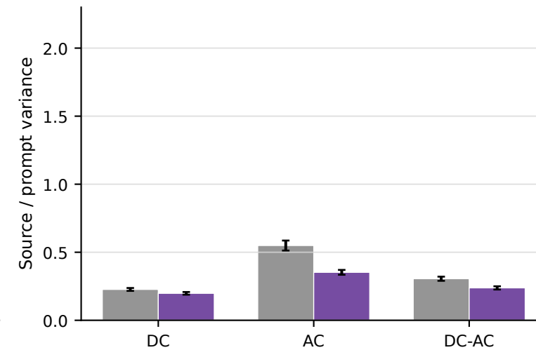
Ministral-3-8B-Instruct-2512
