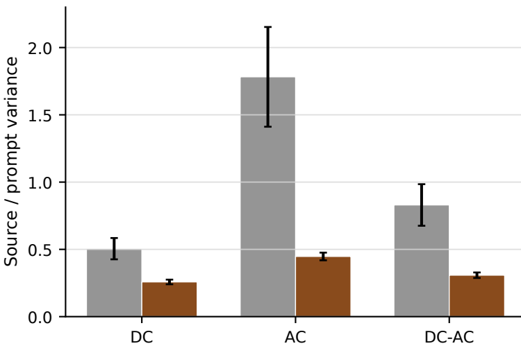
Llama-3.1-8B-Instruct
