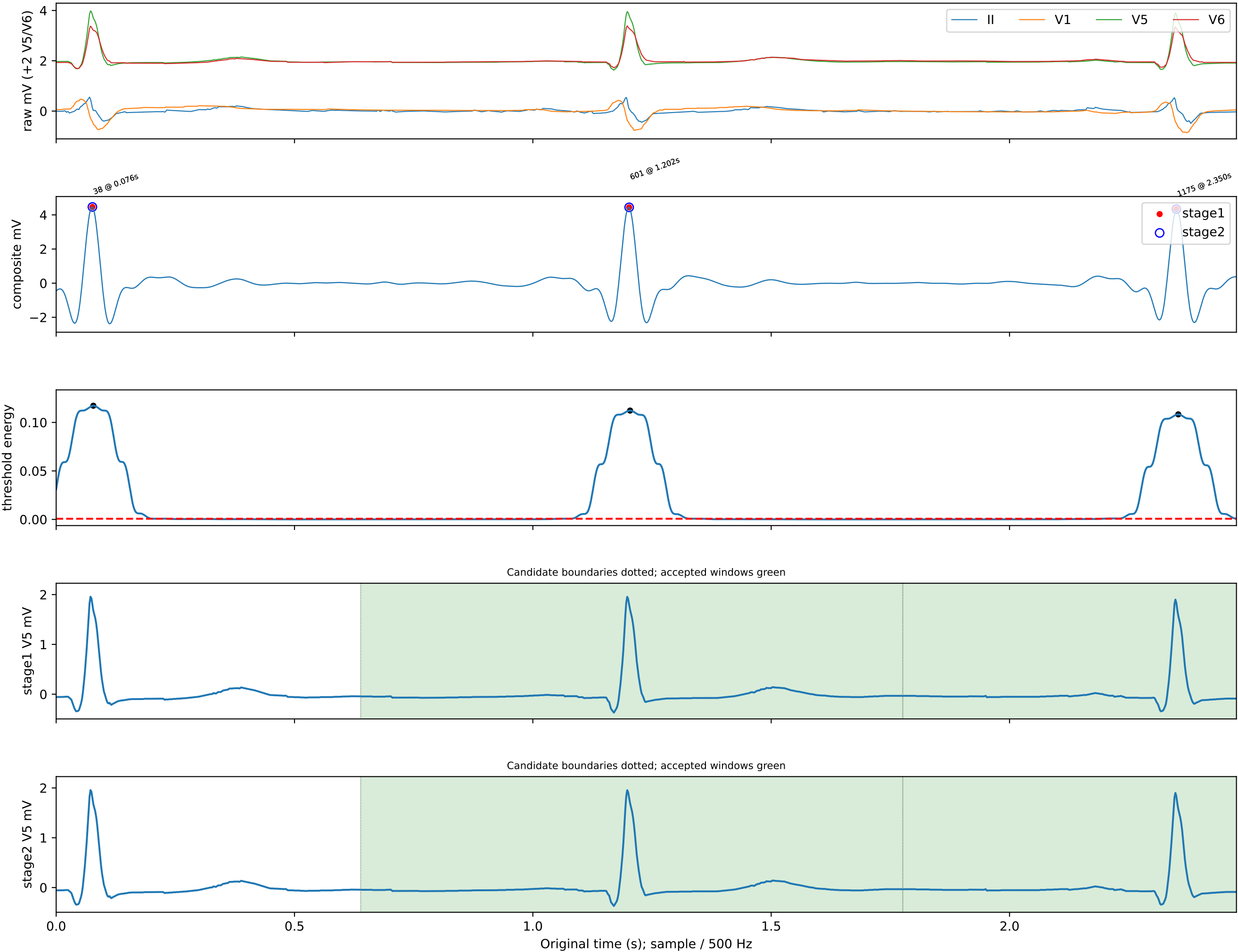
ecg_id=2557 NORM: local inspection 0.00-2.48s; no independent peak annotation
