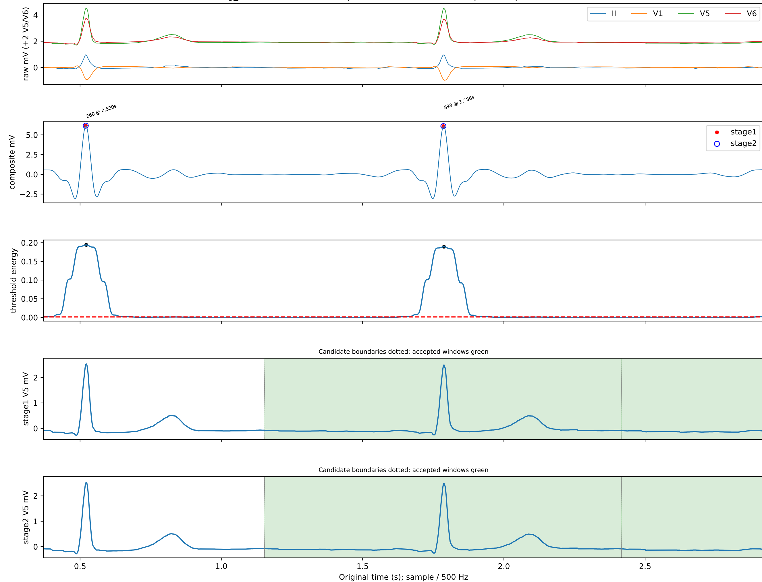
ecg_id=19635 LVH: local inspection 0.37-2.92s; no independent peak annotation
