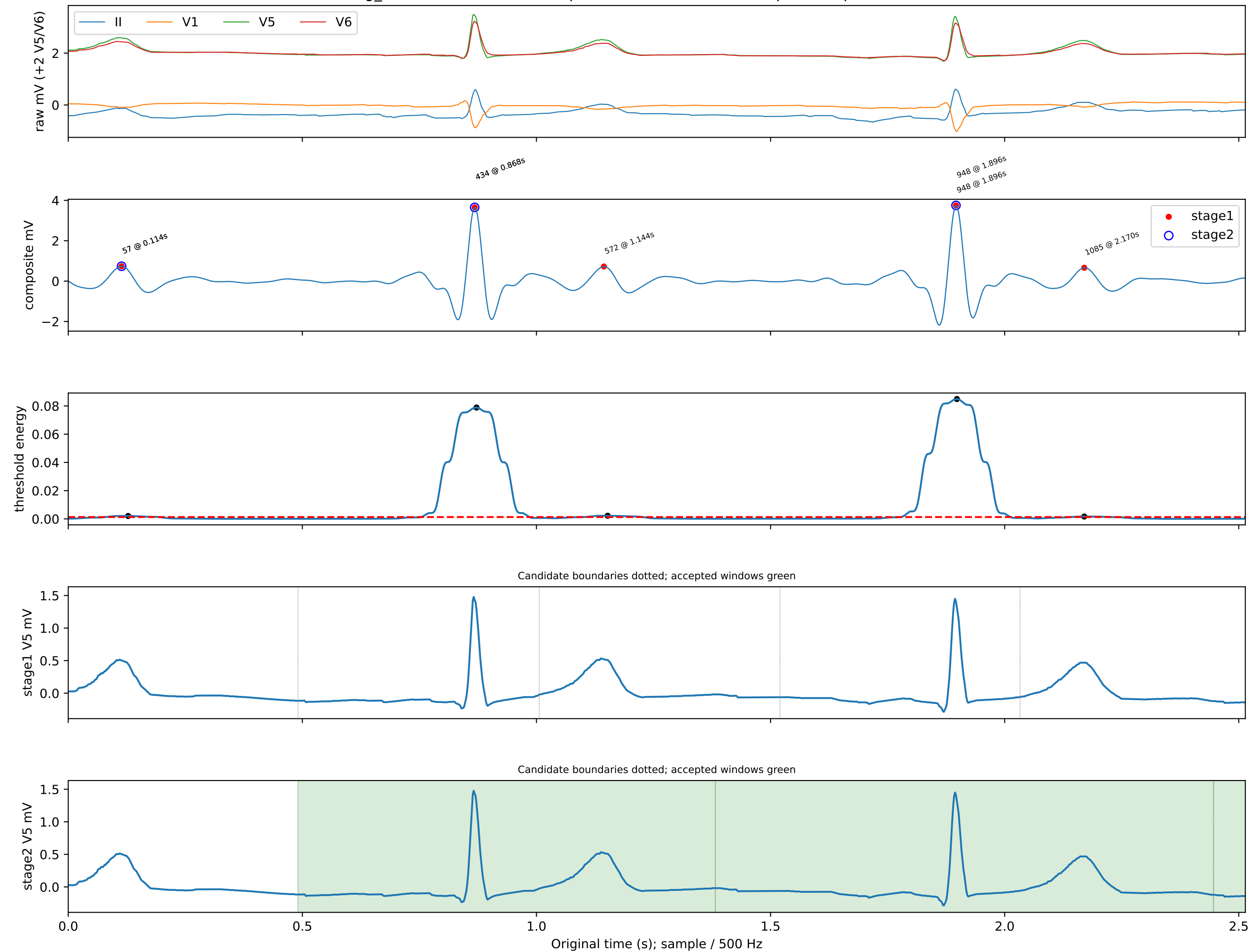
ecg_id=5962 NORM: local inspection 0.00-2.51s; no independent peak annotation
