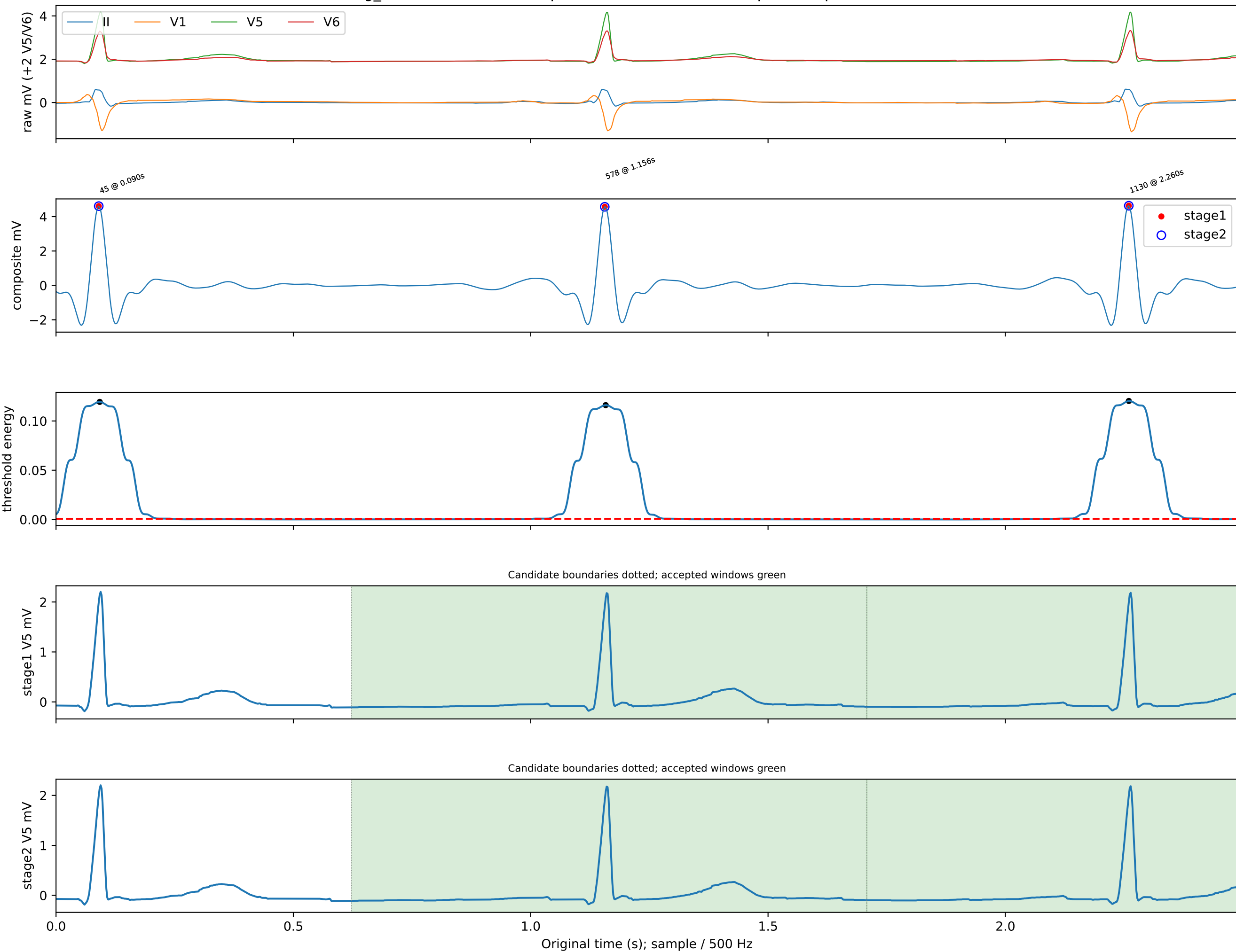
ecg_id=3316 LVH: local inspection 0.00-2.49s; no independent peak annotation
