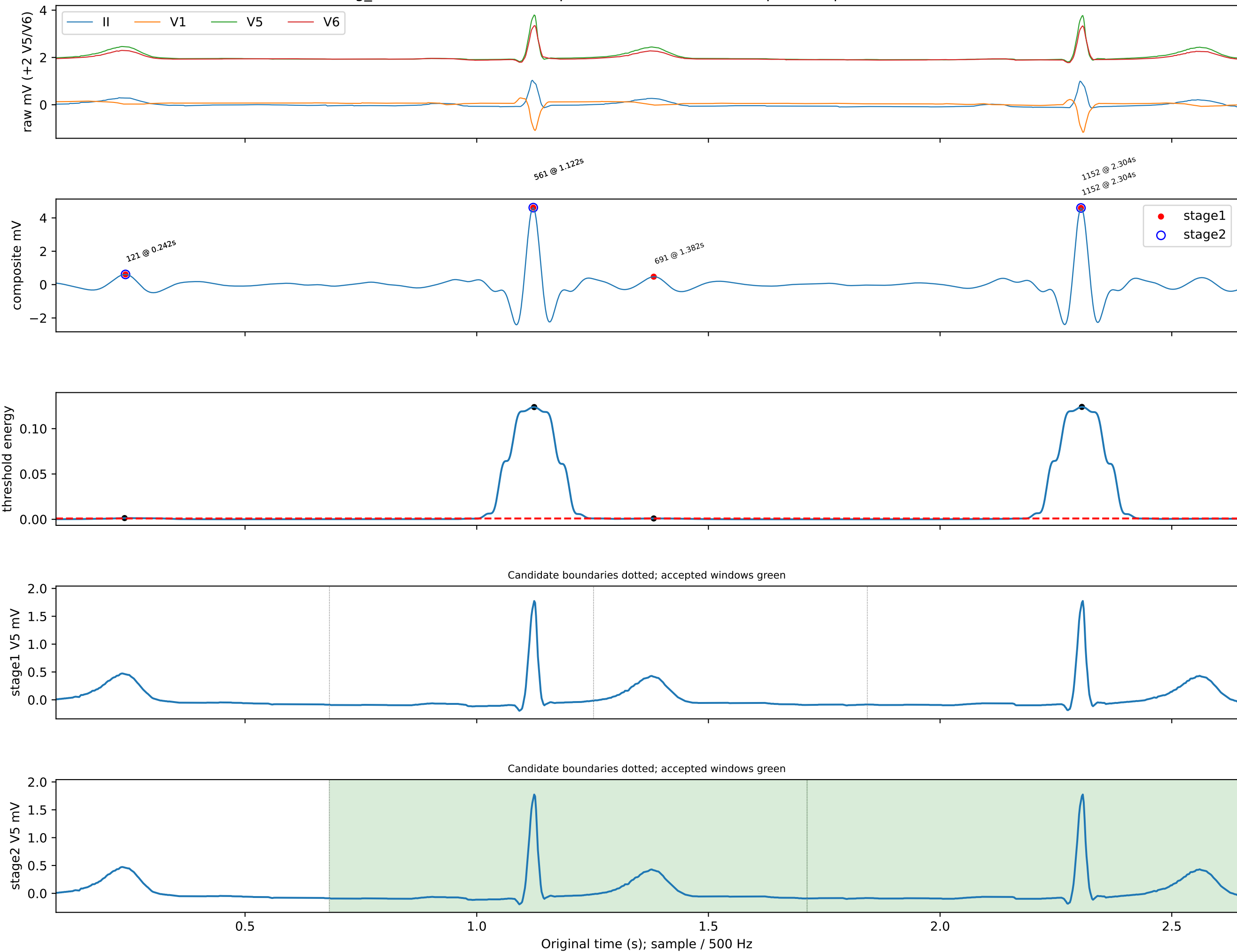
ecg_id=4210 NORM: local inspection 0.09-2.64s; no independent peak annotation
