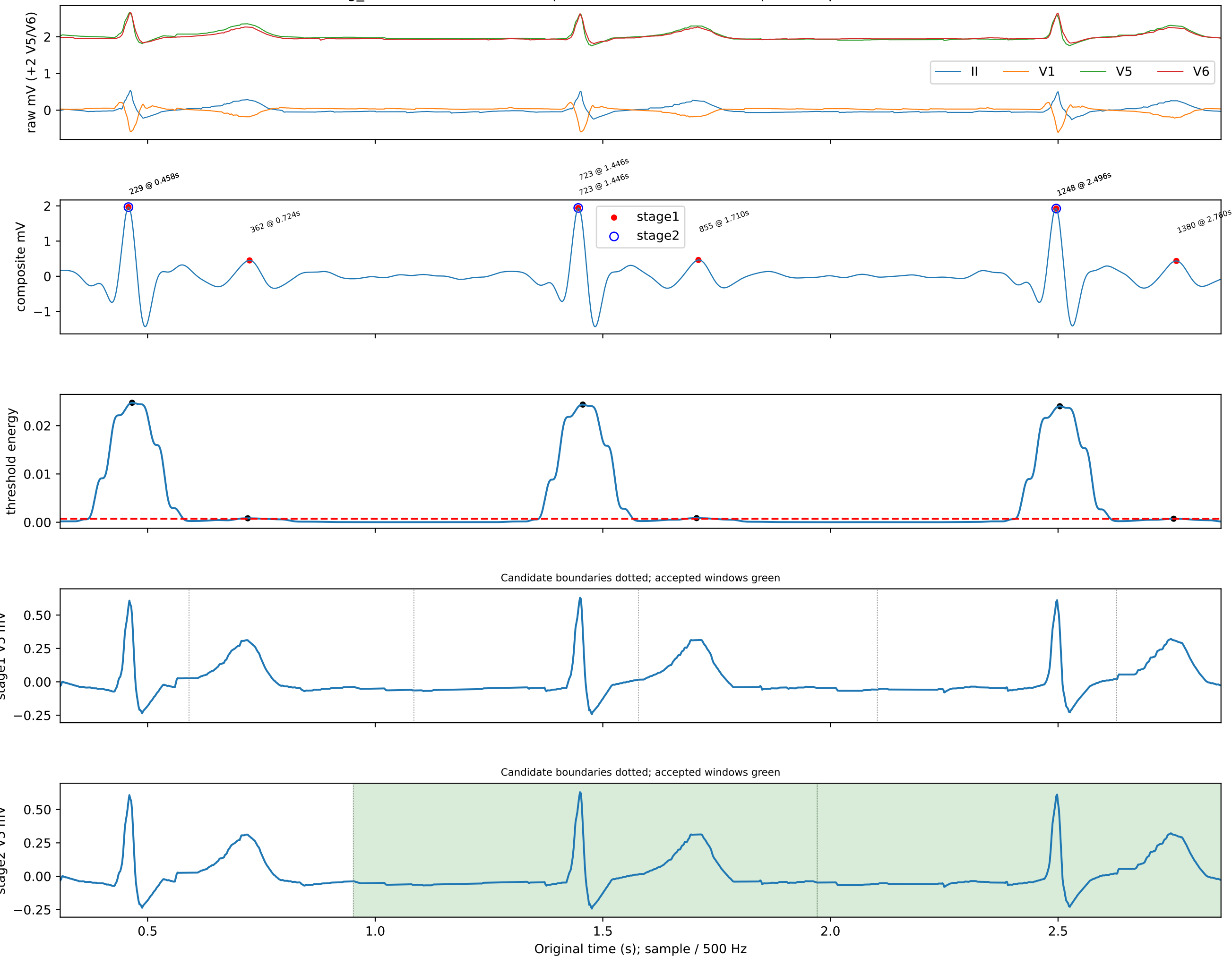
ecg_id=4802 NORM: local inspection 0.31-2.86s; no independent peak annotation
