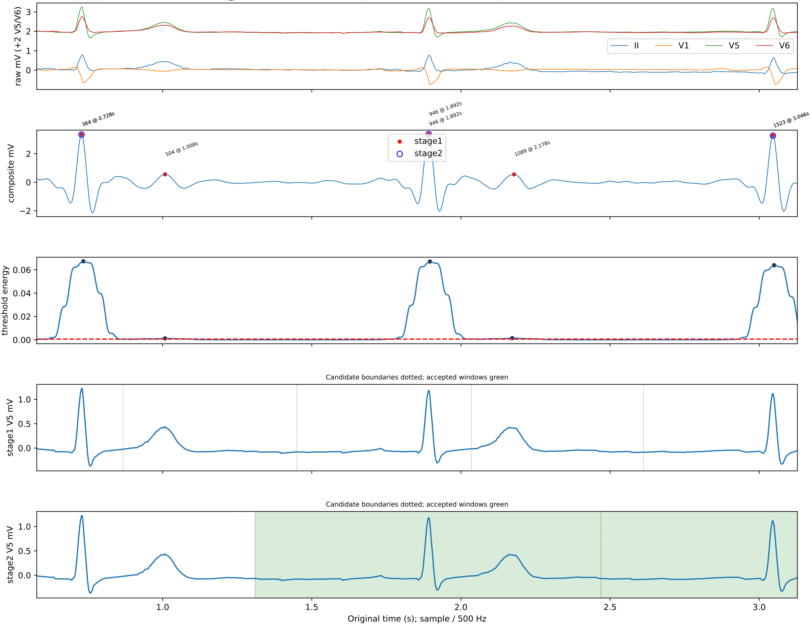
ecg_id=12118 NORM: local inspection 0.58-3.13s; no independent peak annotation
