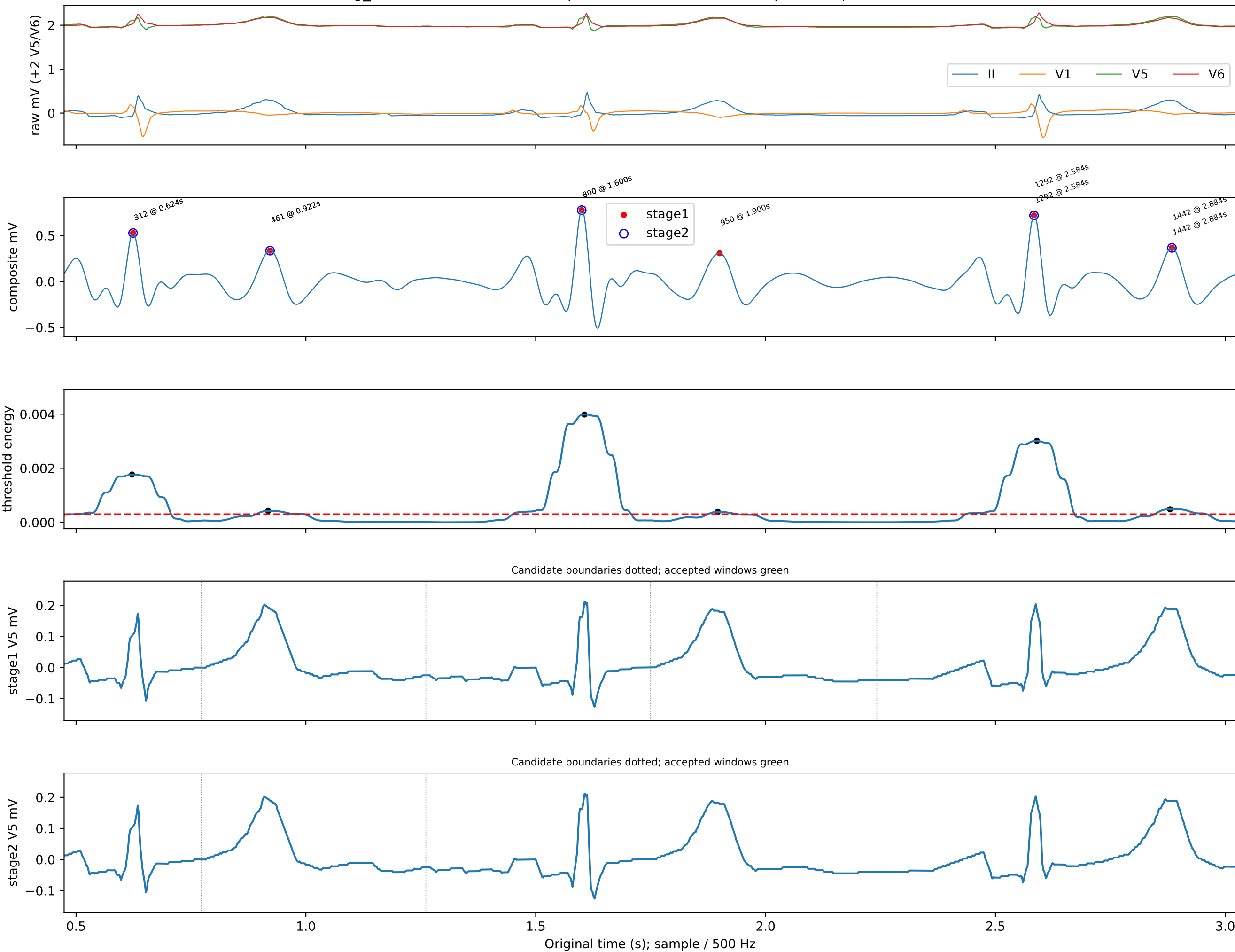
ecg_id=19122 NORM: local inspection 0.47-3.02s; no independent peak annotation
