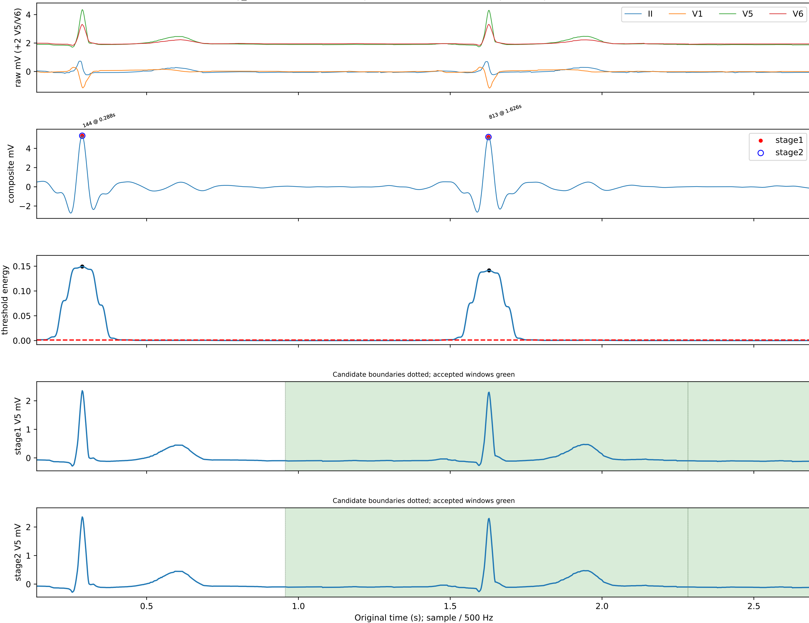
ecg_id=18147 LVH: local inspection 0.14-2.69s; no independent peak annotation
