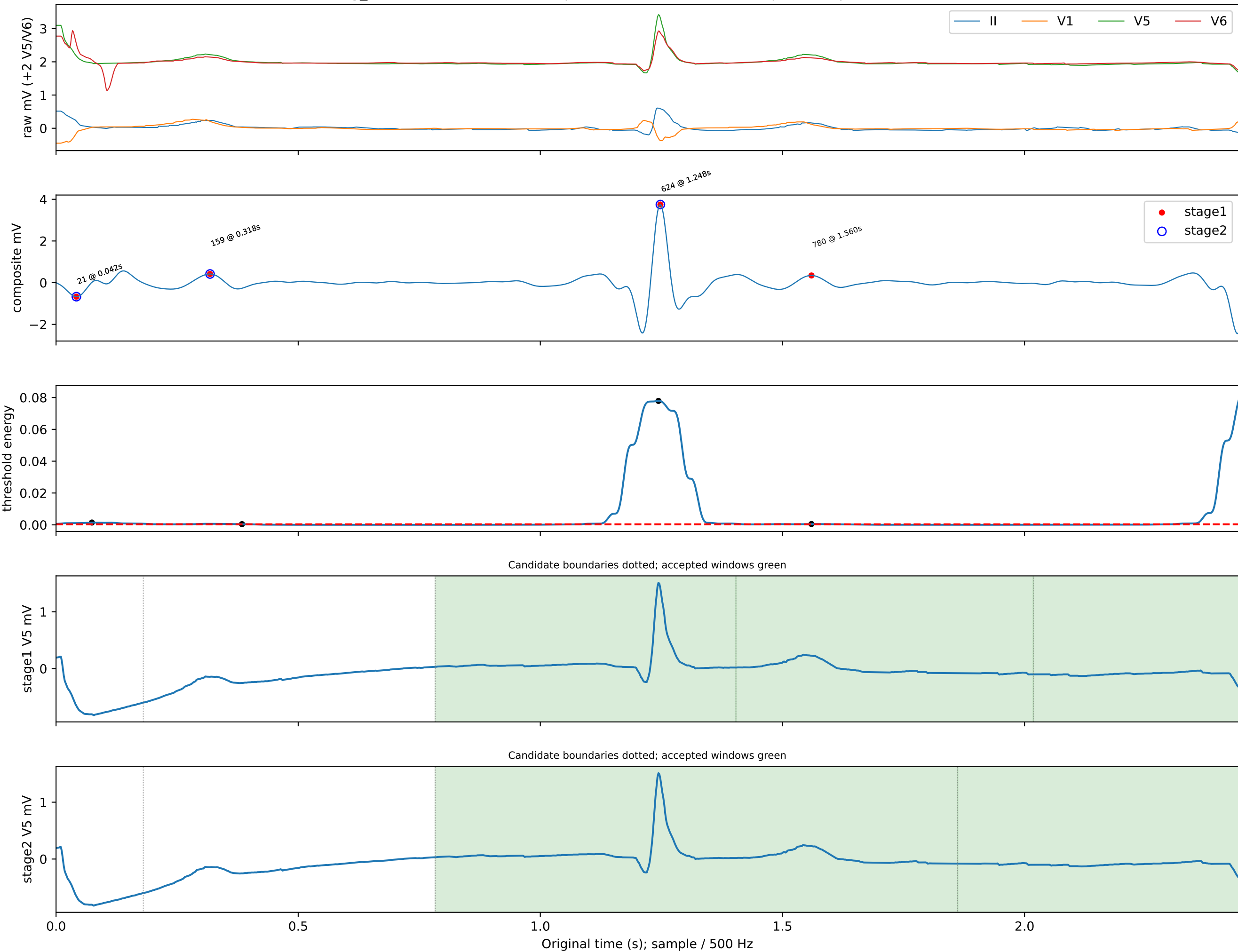
ecg_id=20897 NORM: local inspection 0.00-2.44s; no independent peak annotation
