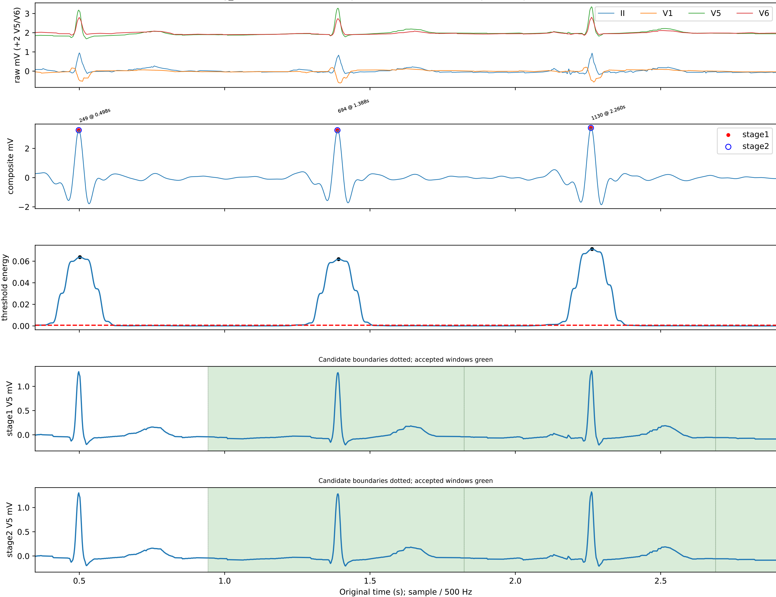
ecg_id=6534 NORM: local inspection 0.35-2.90s; no independent peak annotation
