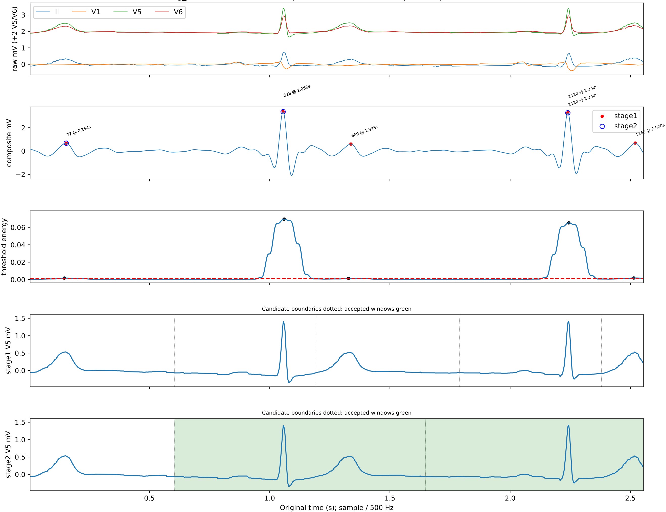
ecg_id=19708 NORM: local inspection 0.00-2.55s; no independent peak annotation
