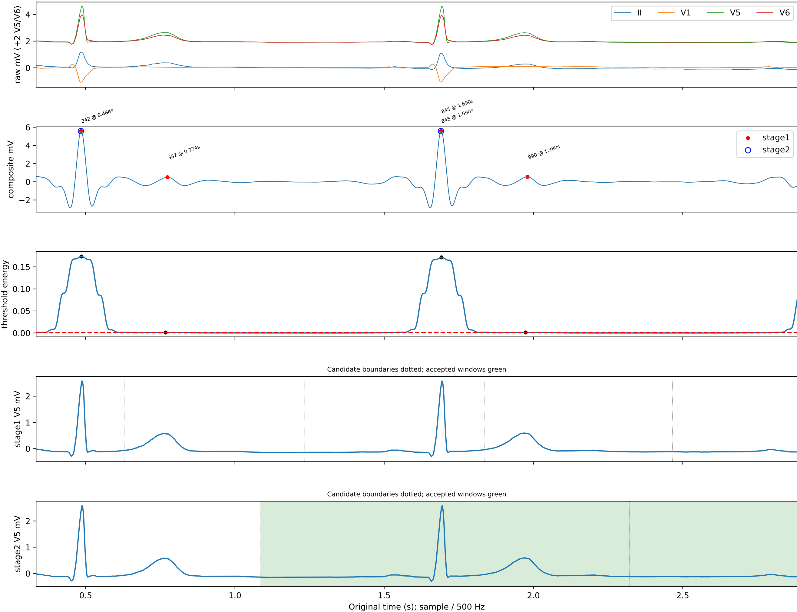
ecg_id=13919 LVH: local inspection 0.33-2.88s; no independent peak annotation
