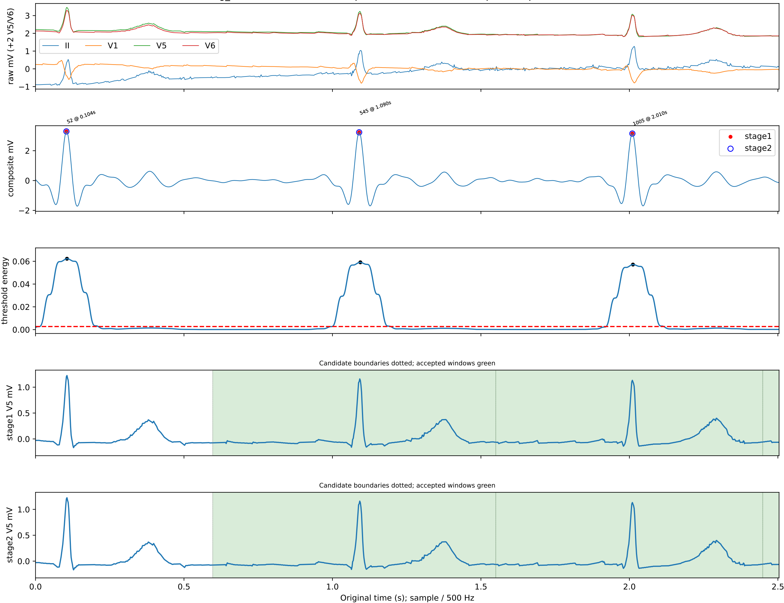
ecg_id=15974 NORM: local inspection 0.00-2.50s; no independent peak annotation
