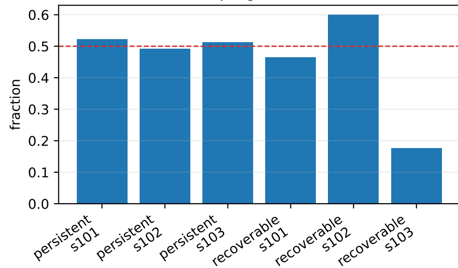
No-progress rate
