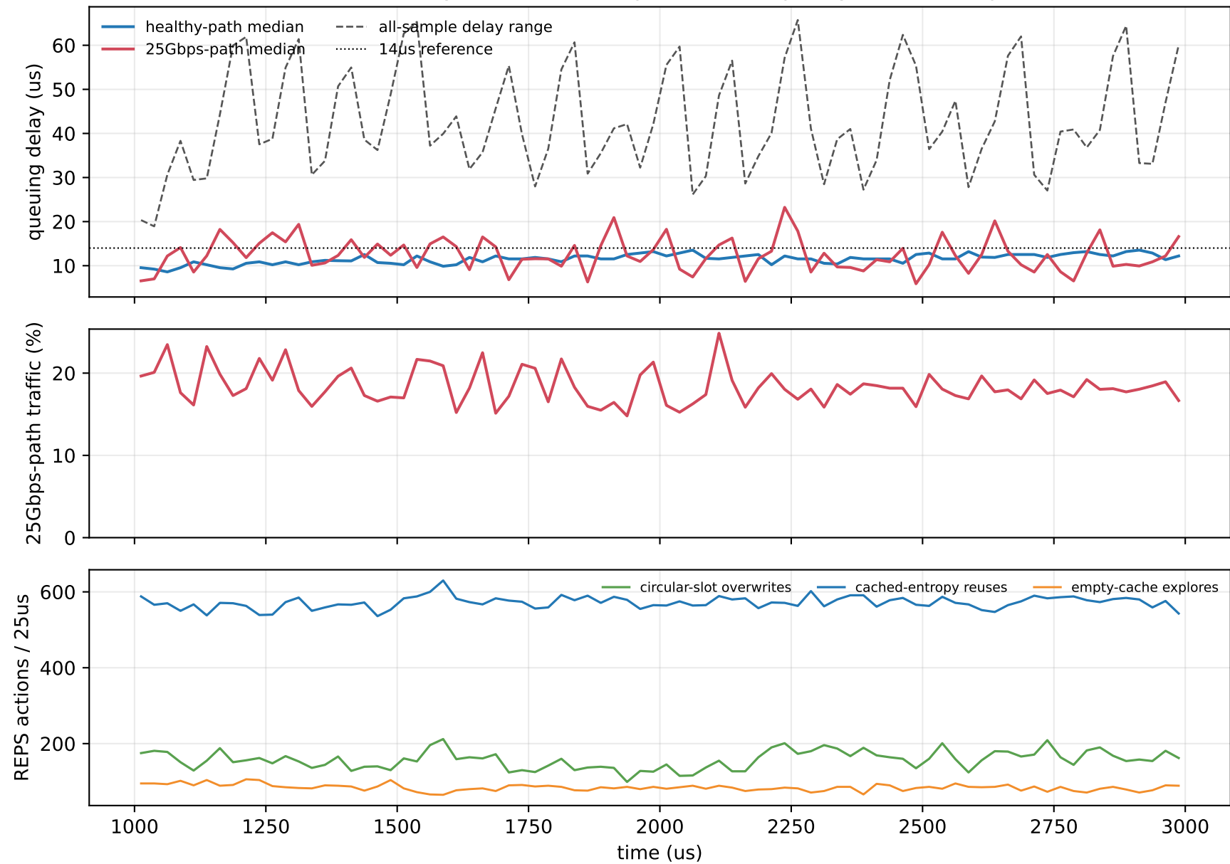
Actual 8-entry REPS + NSCC, persistent capacity case (25Gbps)
