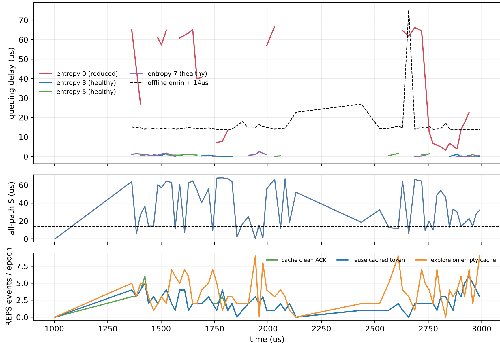
Vanilla REPS + NSCC, recoverable capacity case (25Gbps): flow 1
