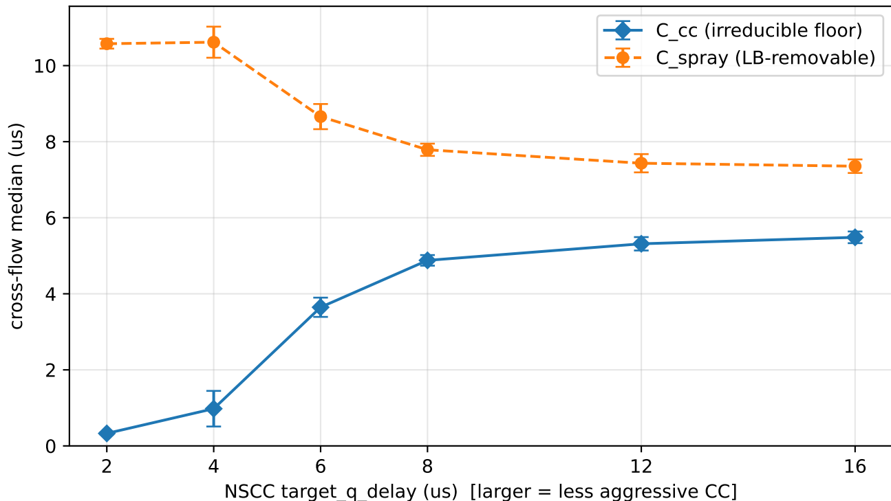
FigF. CC strength sets the floor: C_cc tracks NSCC target_q_delay (REPS, failed=12, high load) -> tightening CC drives the floor toward 0
