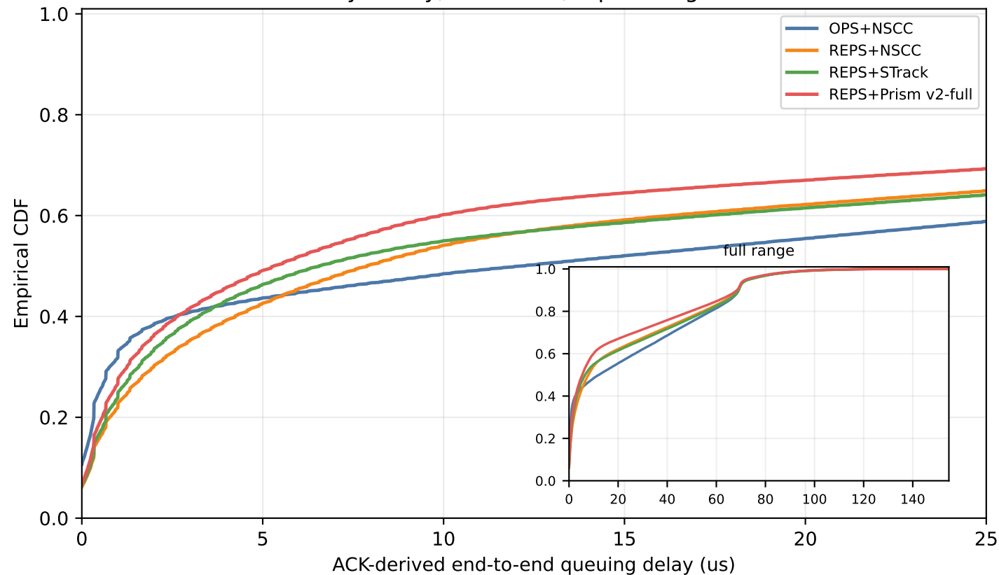
1024-node many2many, failed=16; equal-weight five-seed ECDF
