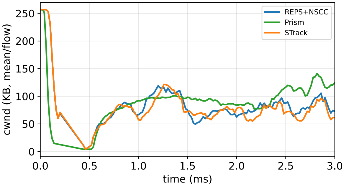
Mechanism @ -failed=8: cwnd
