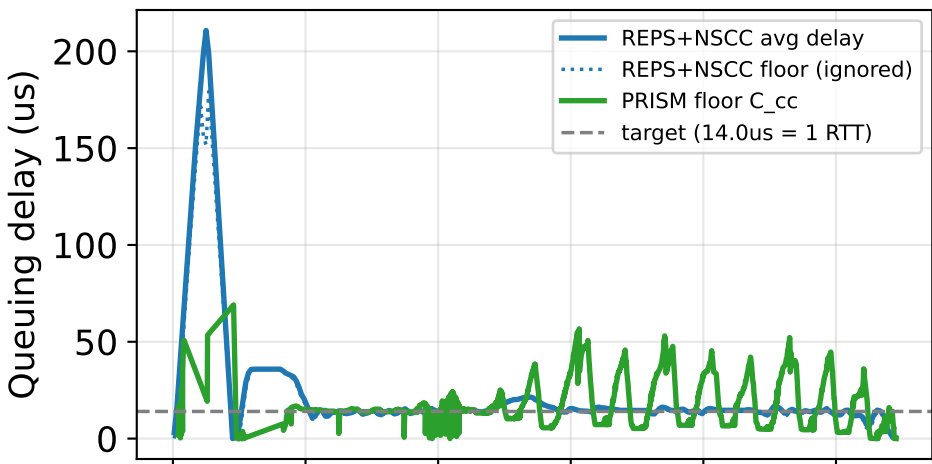
Mechanism @ fan-in=64
