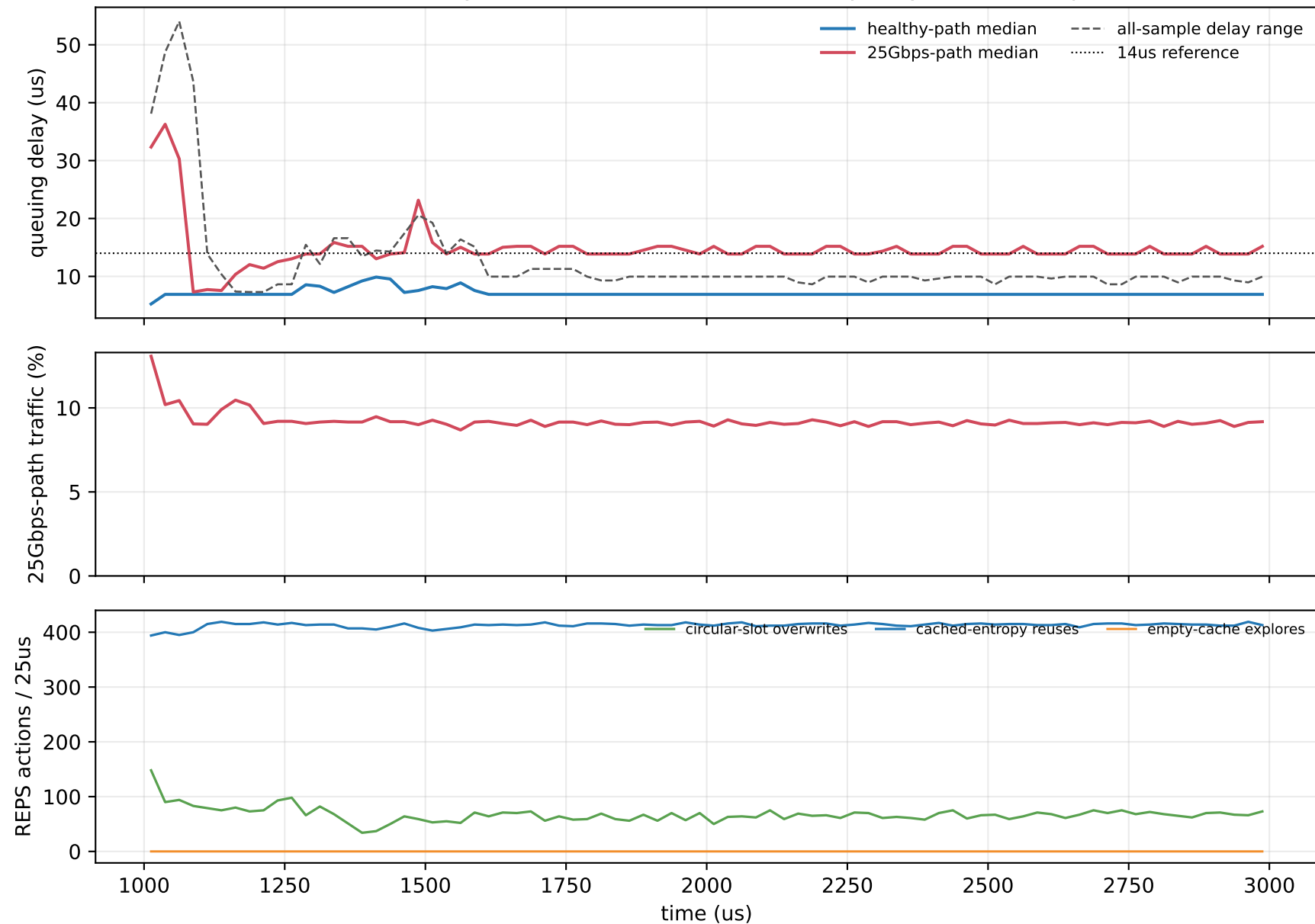
Actual 8-entry REPS + NSCC, recoverable capacity case (25Gbps)
