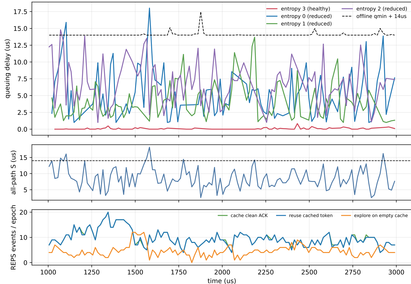
Vanilla REPS, persistent capacity case (25Gbps): flow 1
