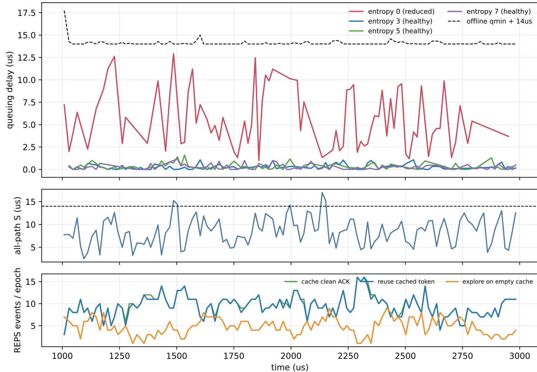
Vanilla REPS, recoverable capacity case (25Gbps): flow 1
