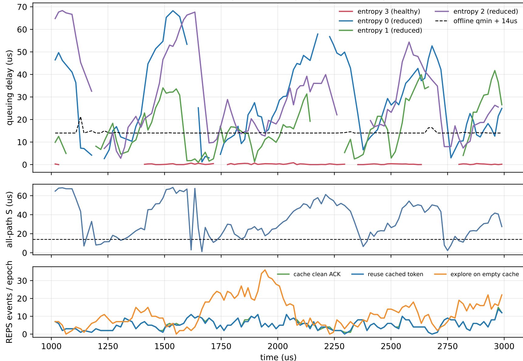
Vanilla REPS + NSCC, persistent capacity case (25Gbps): flow 1
