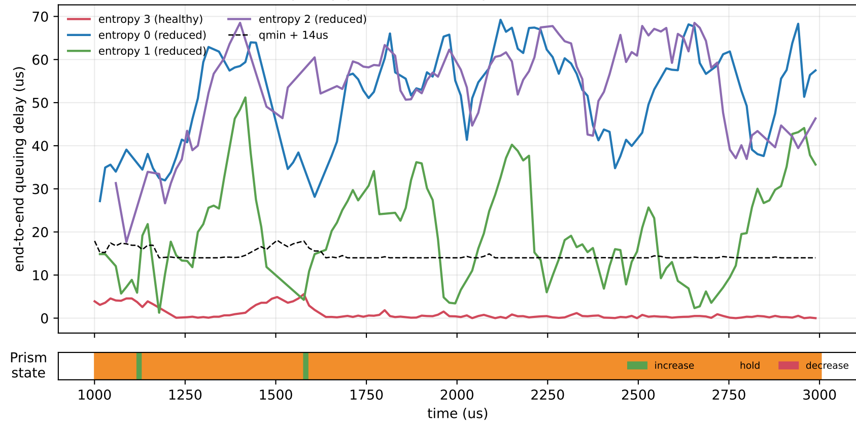
M2 capacity-persistent, 25Gbps reduced links: flow 1
