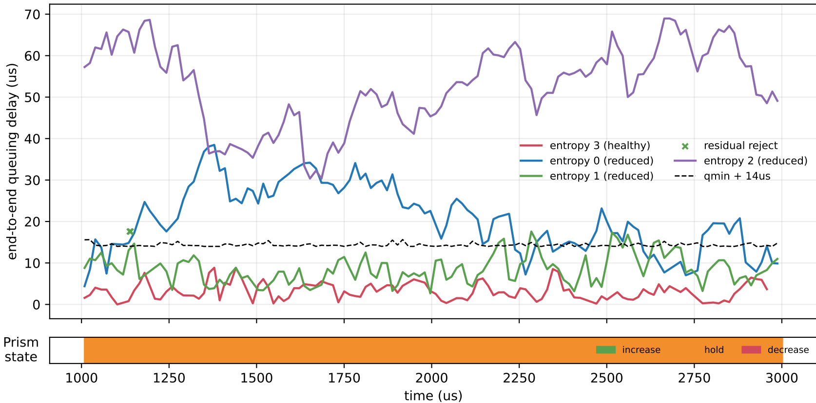
M2 persistent: representative paths of flow 1
