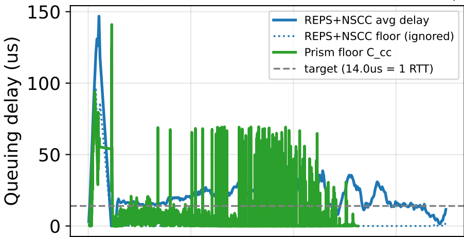
Mechanism @ 4:1 oversub (100G), failed=4 (cr=1 win point)
