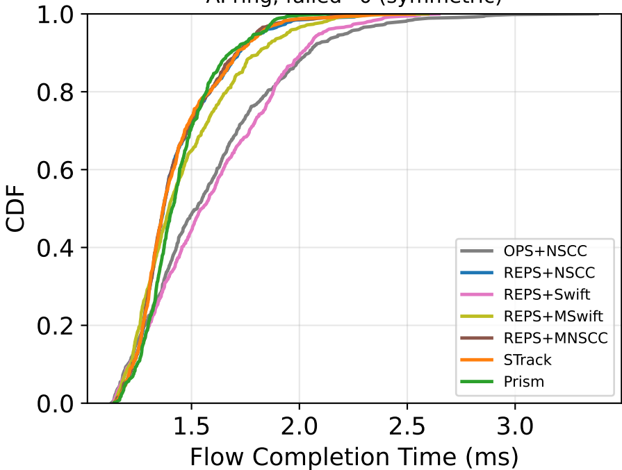
Al ring, failed=0 (symmetric)
