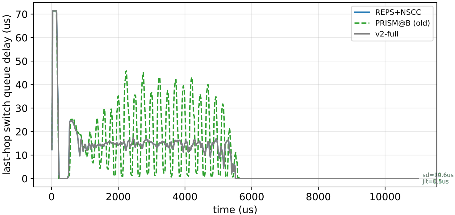
queue stability — incast n32 f=8 (time-series run, seed 13)
