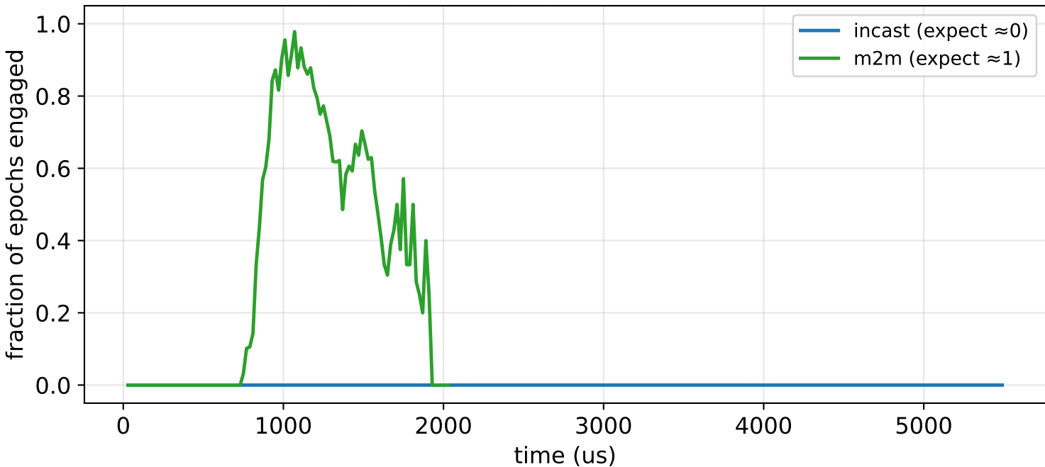
PRISM v2 engage-gate: engaged fraction over time (seed 13)
