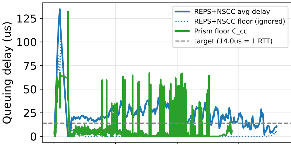
Mechanism @ 4:1 oversub, failed=8 (2/32 core links degraded)
