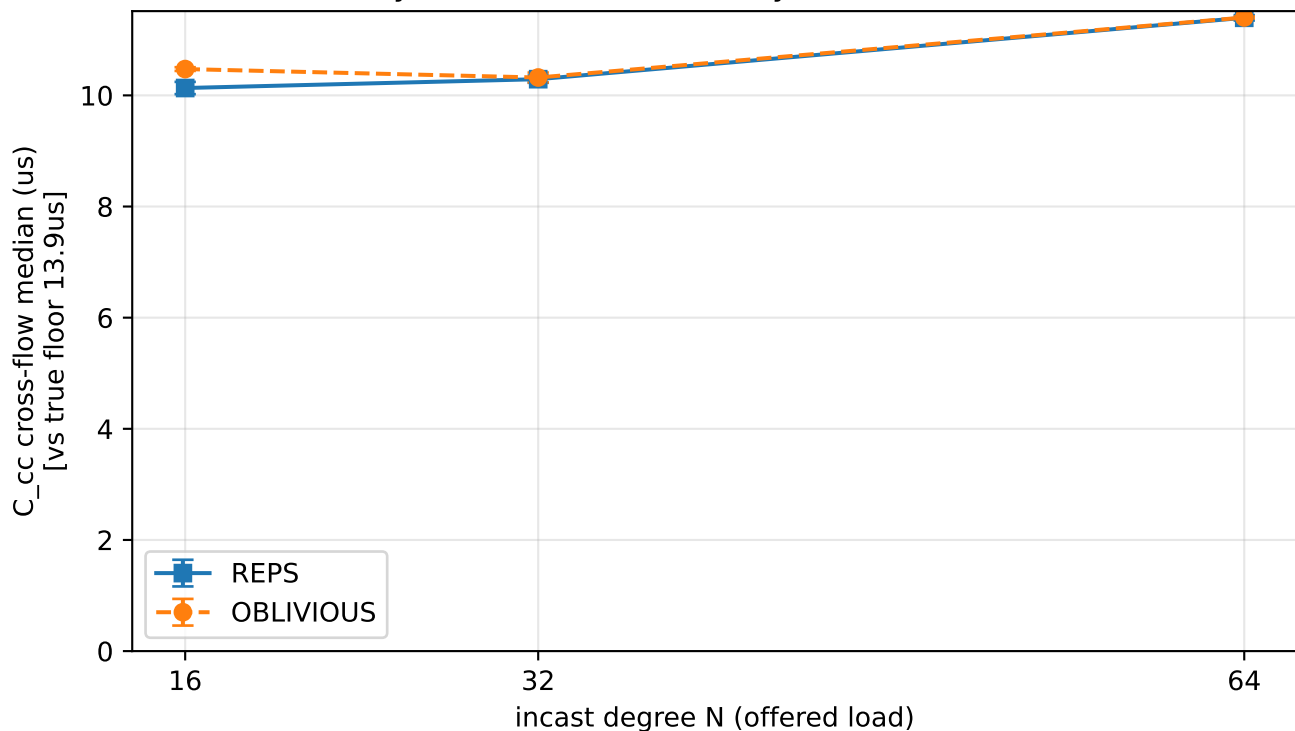
FigA. Irreducible floor C_{cc} rises with load and is LB-invariant (symmetric incast) -> only CC can reduce it
