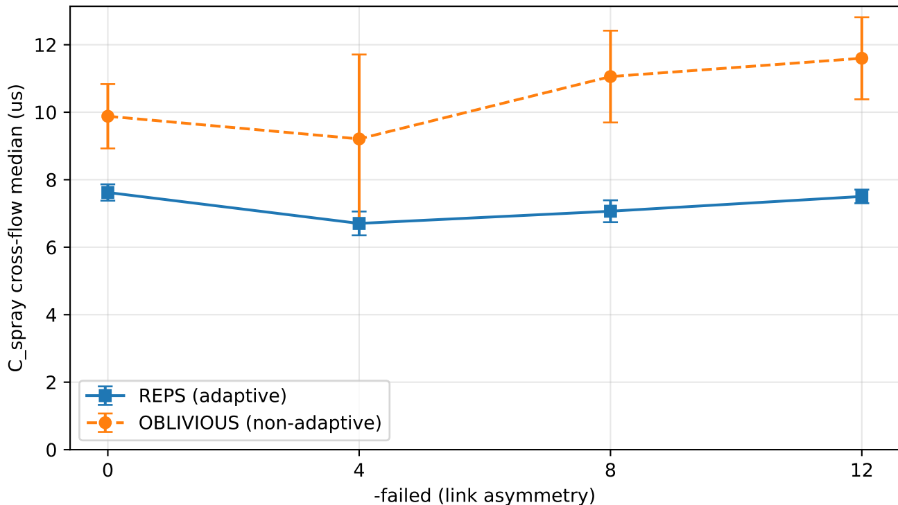
FigB. Removable spread C_spray: good LB lowers it (REPS < OBL) (whole-pod overload, path-diverse) -> spraying/LB is necessary
