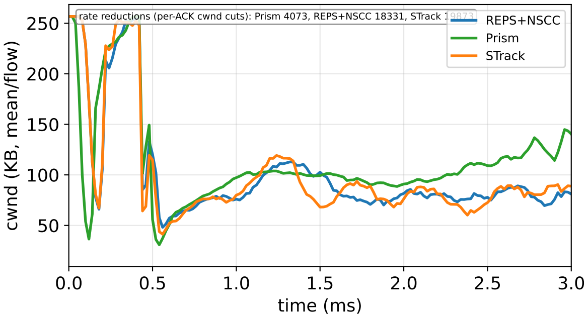
Mechanism @ 1:1, failed=32 (50% pod0 ingress): cwnd
