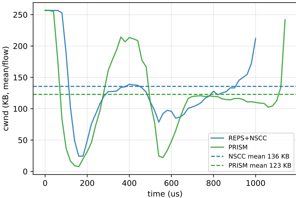
cwnd(t) @ -failed=0 (symmetric): PRISM under-grows
