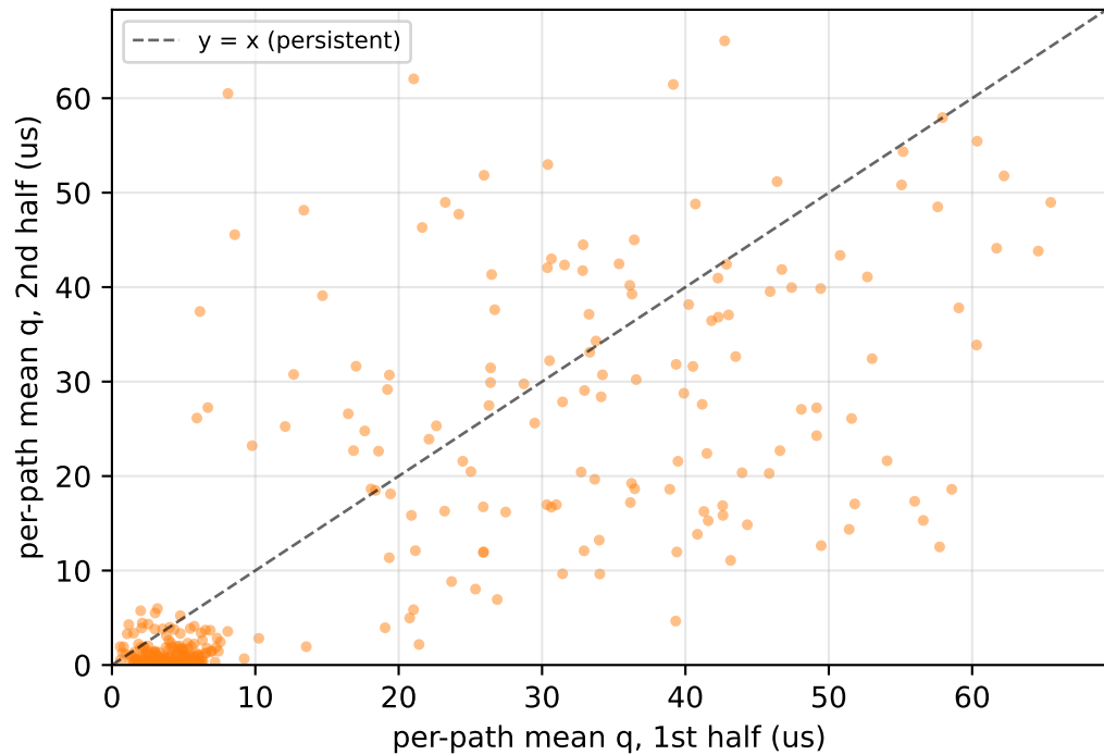
f8 (asymmetric): spread PERSISTS (structural) cross-path spread 32->47us (1st->2nd half)
