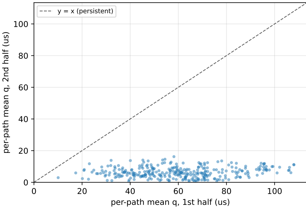
f0 (symmetric): spread is a startup TRANSIENT cross-path spread 31->8us (1st->2nd half)
