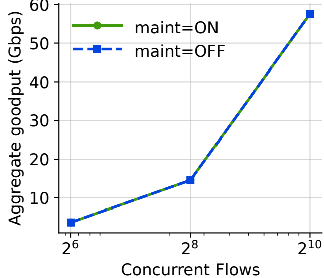
(c) Network goodput
