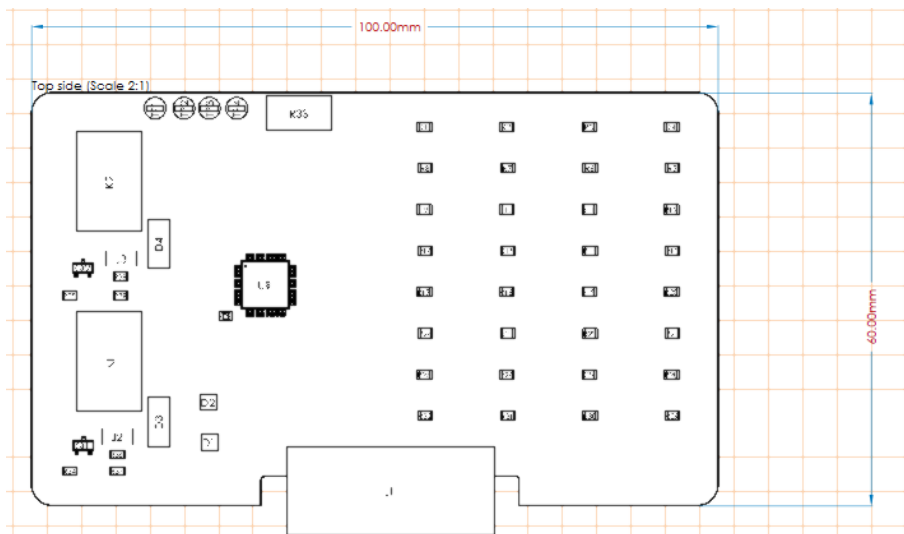
Figure 30 - PCB fille
