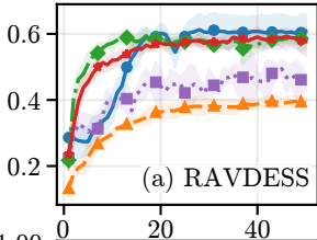
Test accuracy
