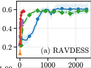
Test accuracy
