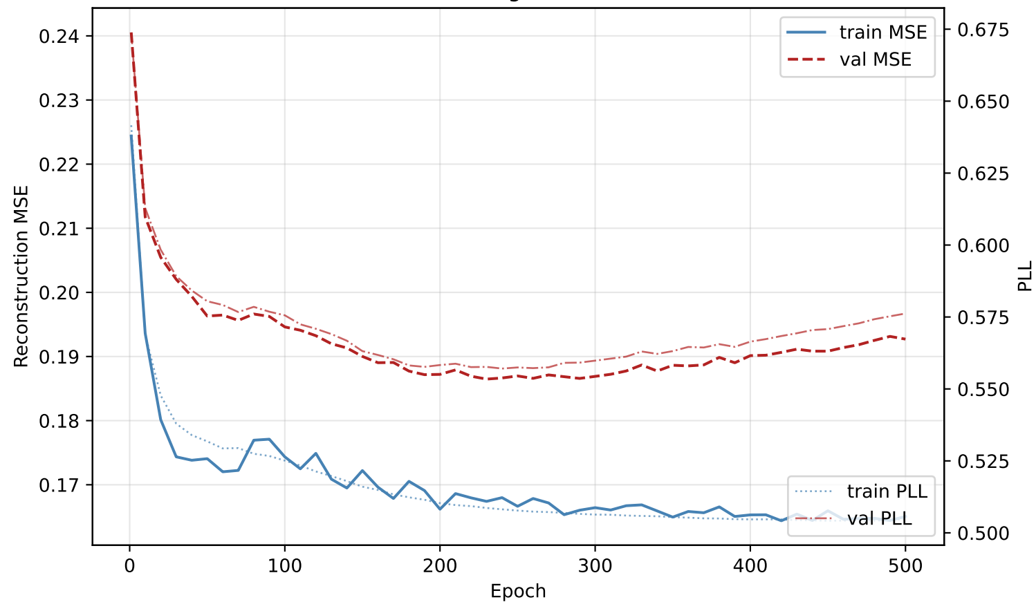
Training curves
