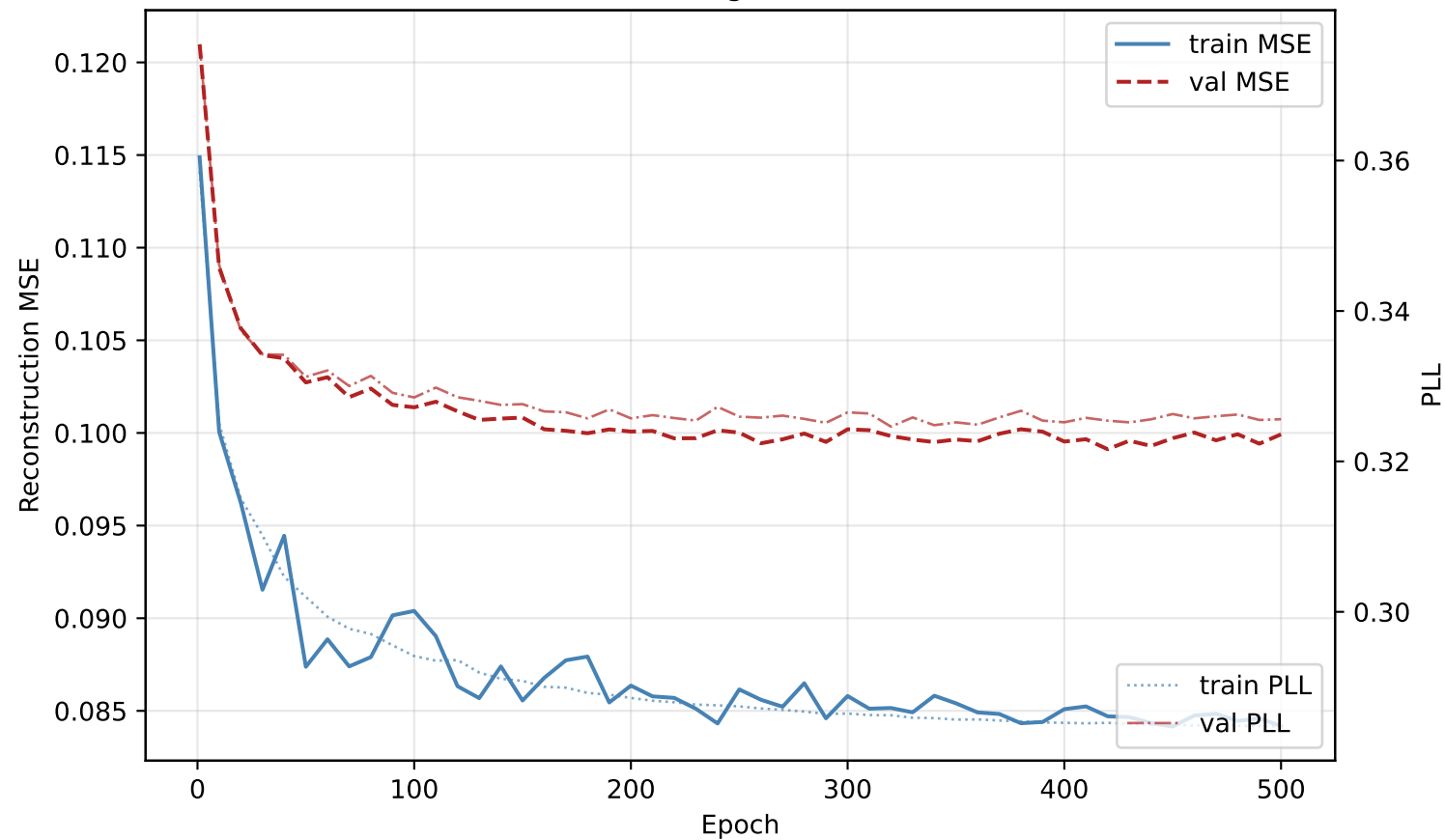
Training curves
