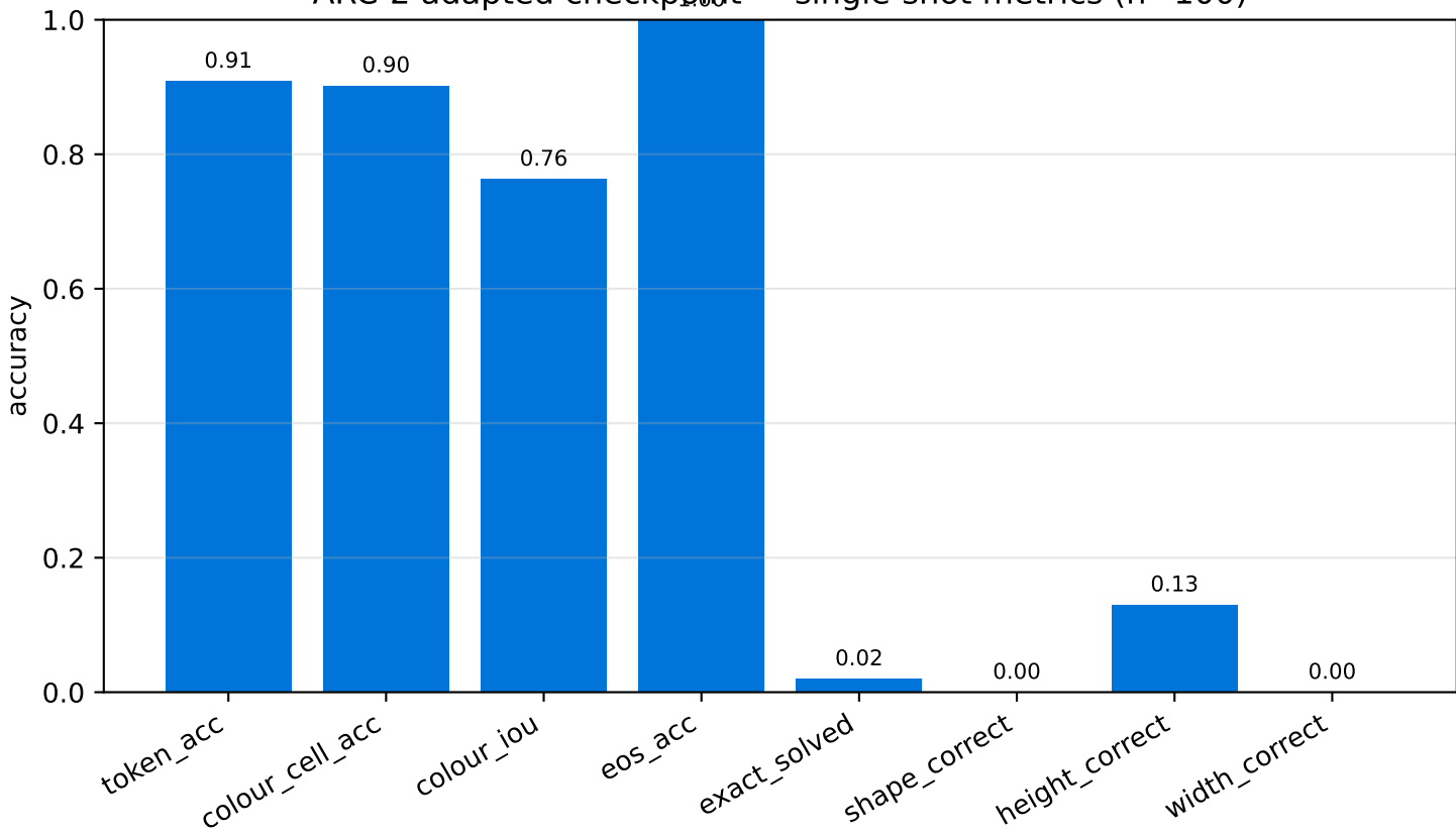
ARC-2 adapted checkpoint — single-shot metrics (n=100)
