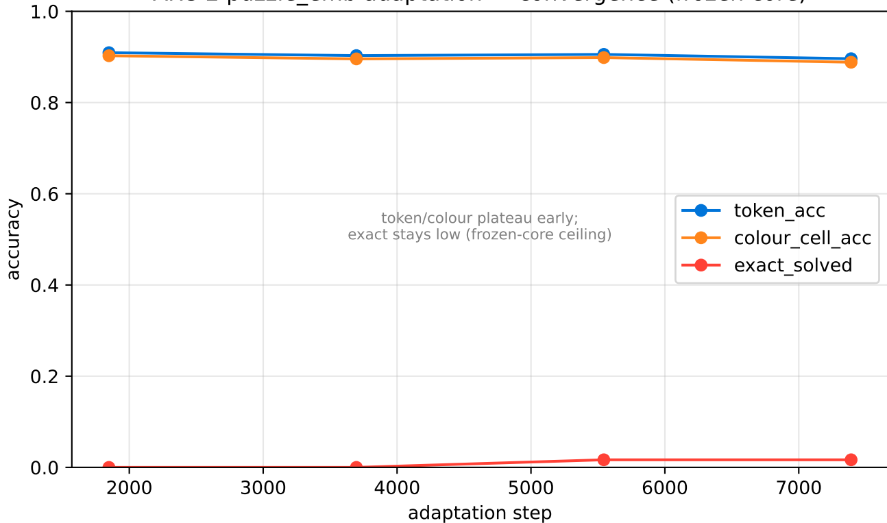
ARC-2 puzzle_emb adaptation — convergence (frozen core)
