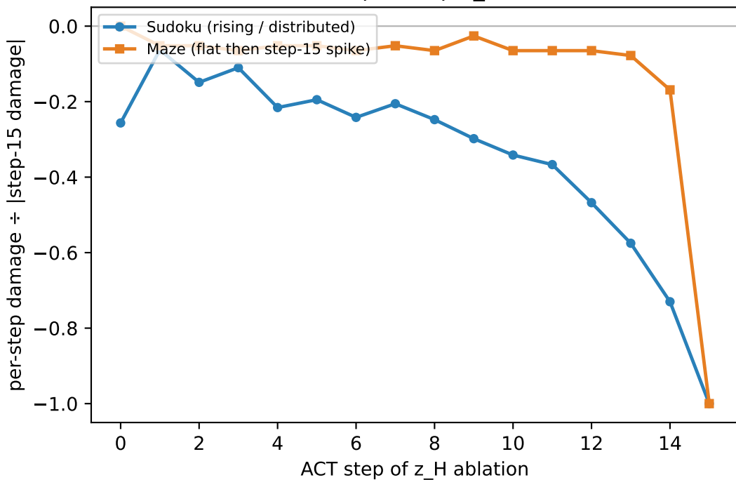
Task-dependent depth: where z_H damage accumulates (normalized per-step z_H ablation)
