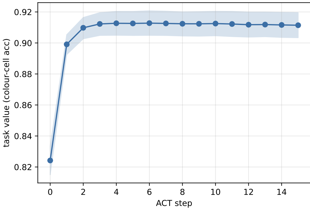
ARC value by reasoning step (policy improvement)
