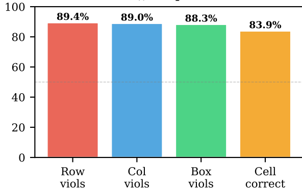
(a) Linear probe readout ( z_H , step 15)
