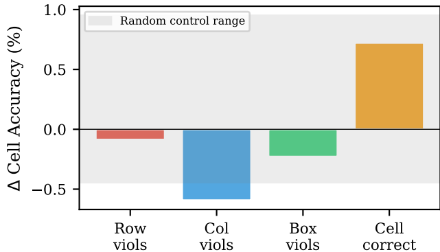
(b) Directed ablation (causal effect)
