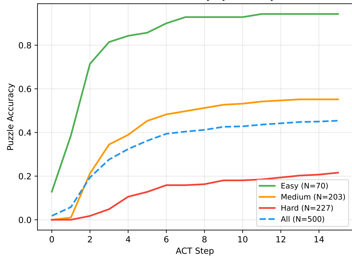
(d) Step 0→15 Improvement by Difficulty
