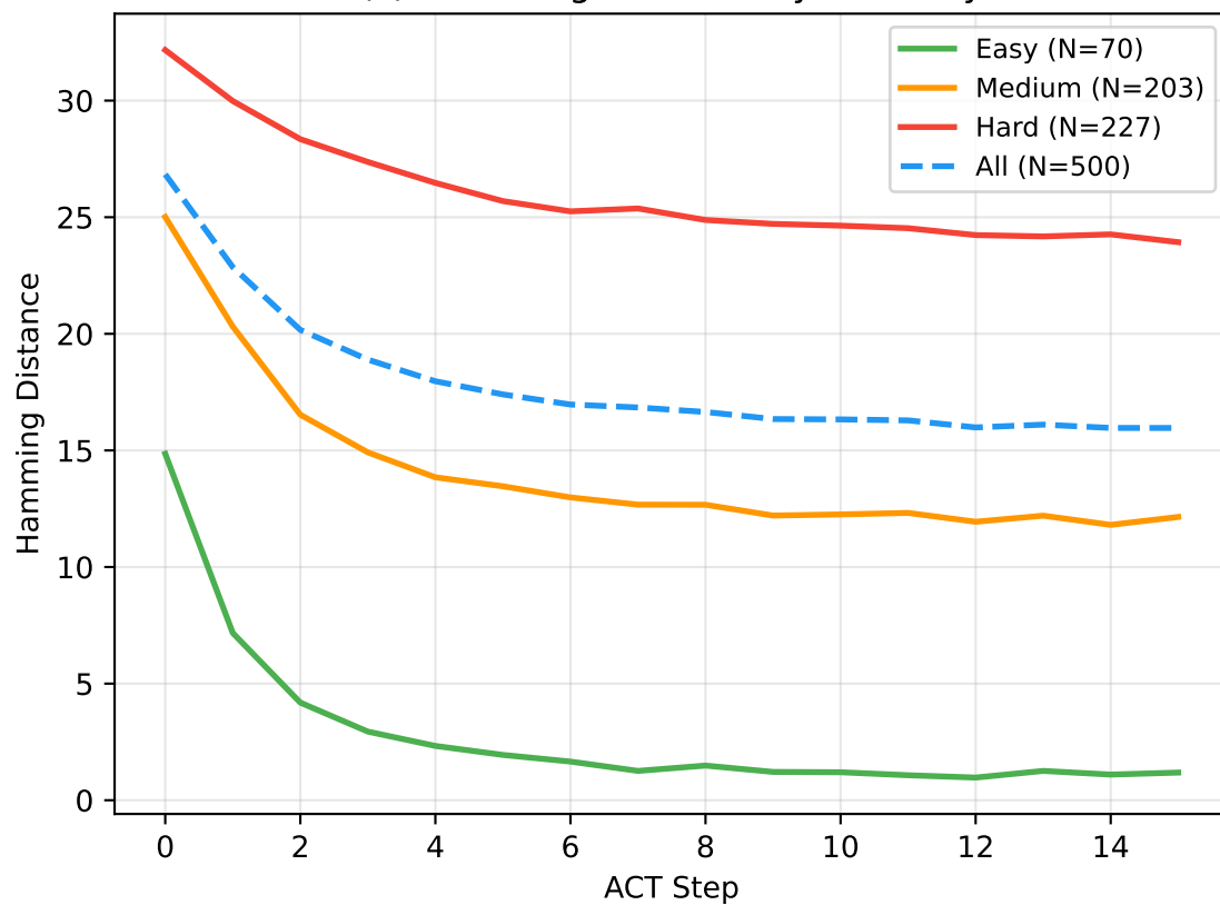
(c) Hamming Distance by Difficulty
