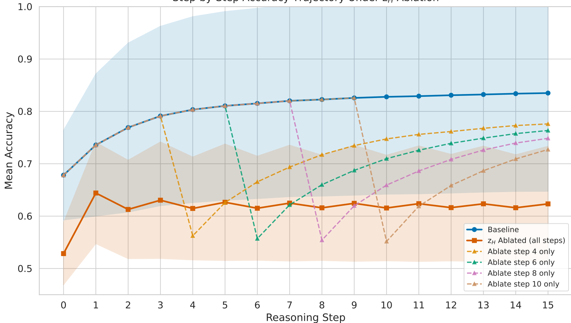
Step-by-Step Accuracy Trajectory Under z_H Ablation
