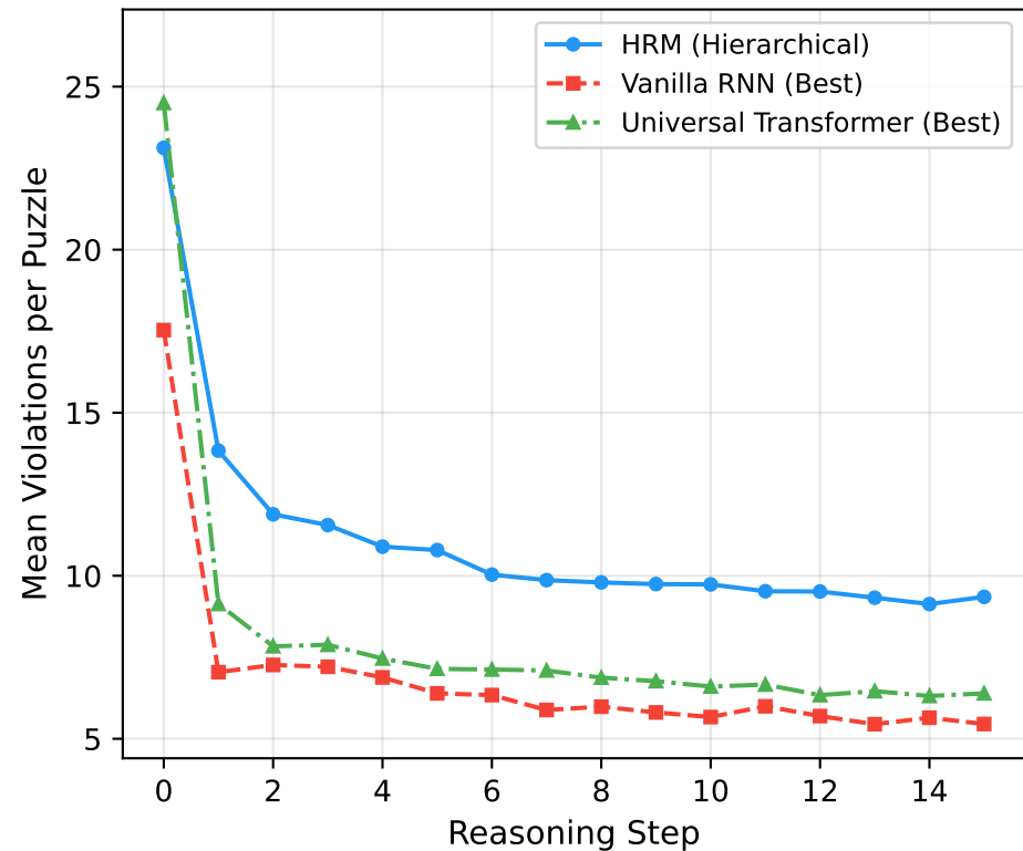
Row Violations
