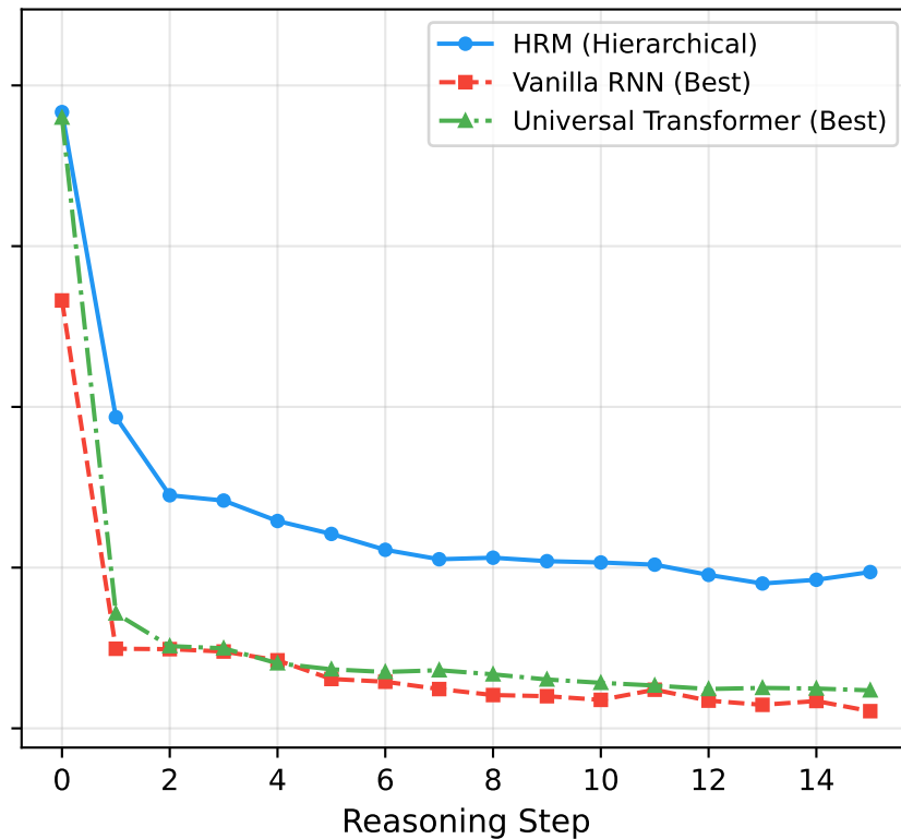
Column Violations
