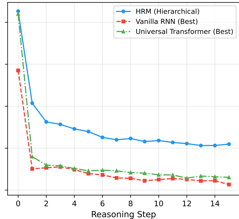
Box Violations
