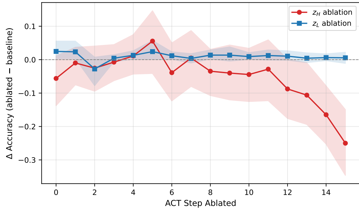
Single-Step Zero Ablation: z_H vs z_L
