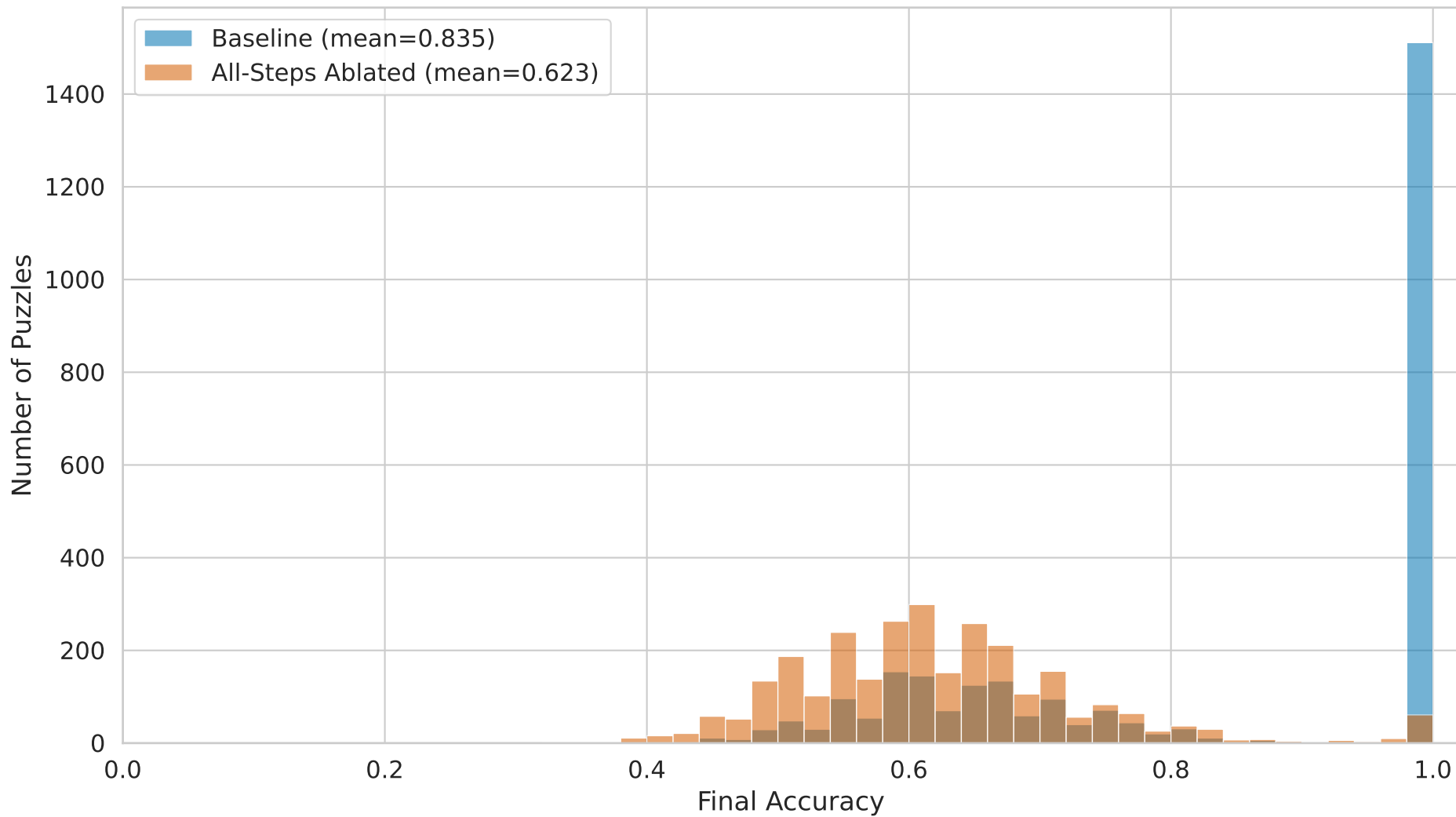
Accuracy Distribution: Baseline vs z_H All-Steps Ablation
