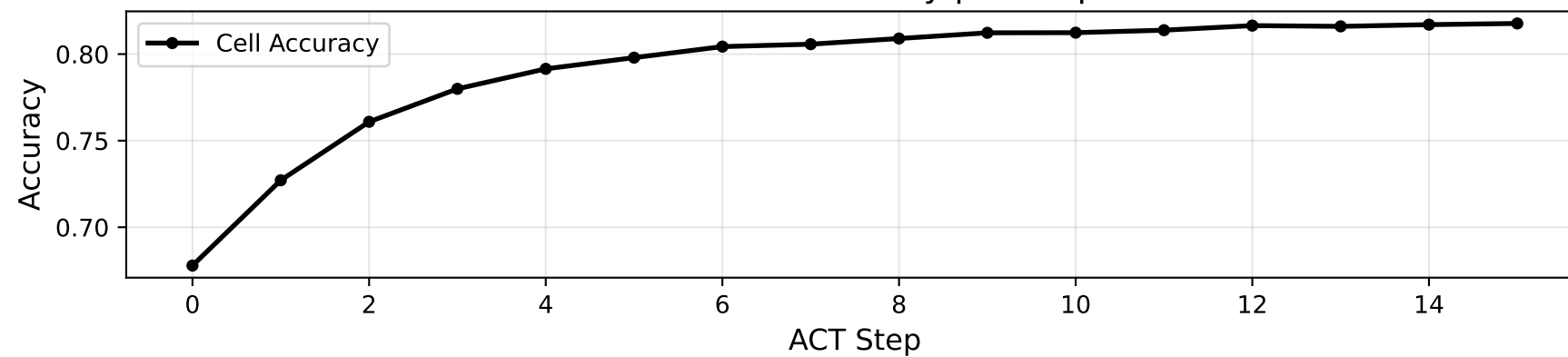
Mean Cell Accuracy per Step
