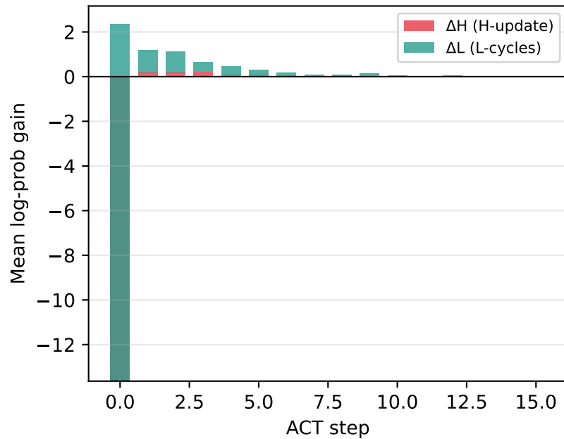
\Delta H + \Delta L breakdown (sudoku)
