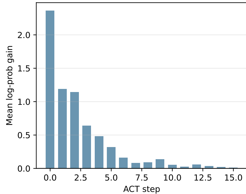
\Delta_{\text{total}} per step (sudoku, solved)
