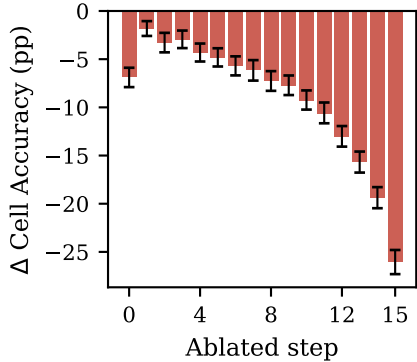
(a) Per-step z_H ablation
