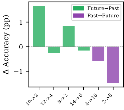
(c) Time-shift transplant
