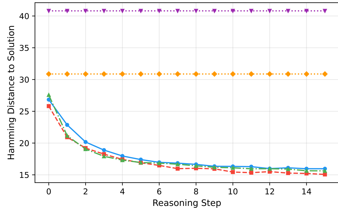
(a) Hamming Distance vs. Step
