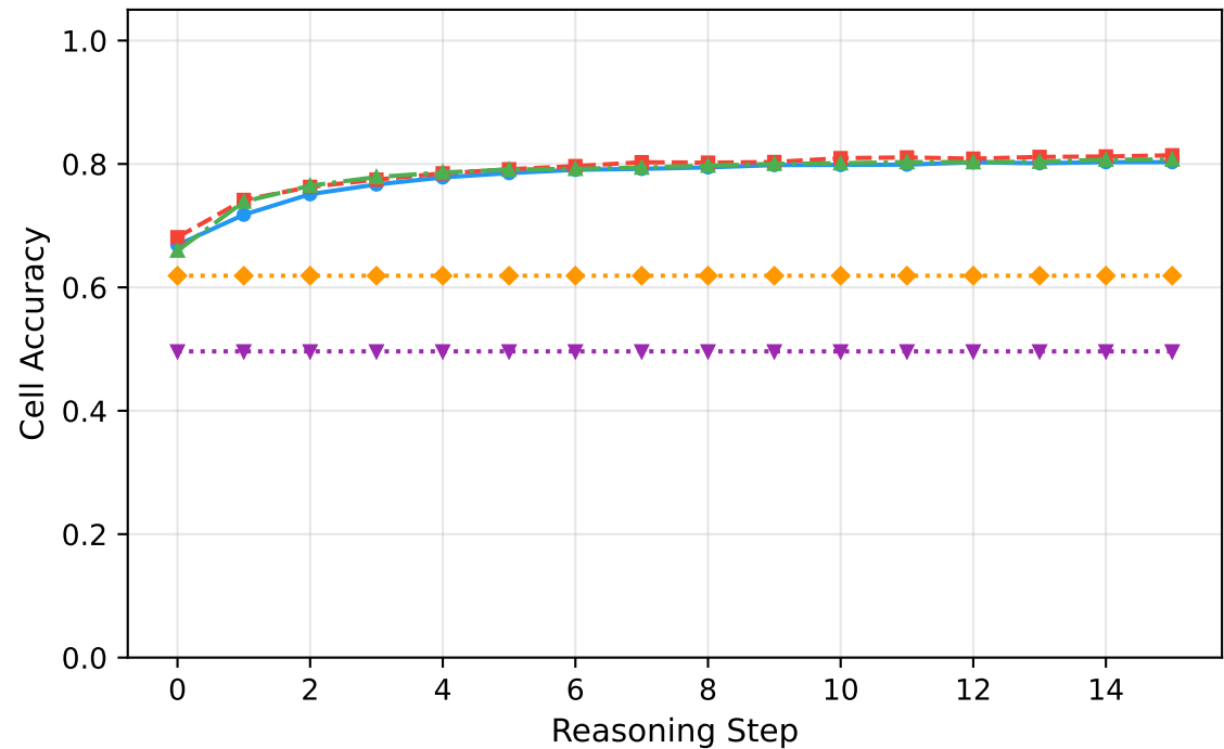
(b) Cell Accuracy vs. Step
