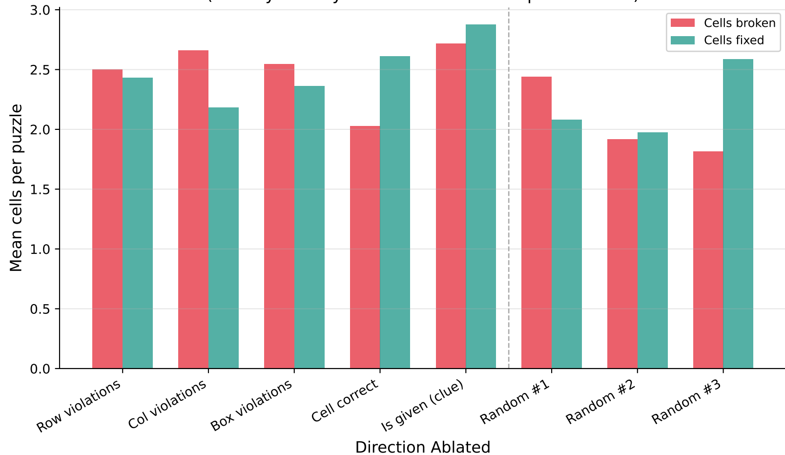
E9: Cells Broken vs Fixed by Directional Ablation (near-symmetry indicates non-causal perturbation)
