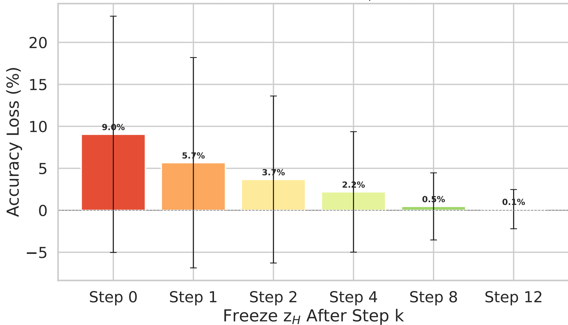
E2-FREEZE: How Much Does Freezing z_H Hurt? (Baseline = 82.0%, n = 200 puzzles)
