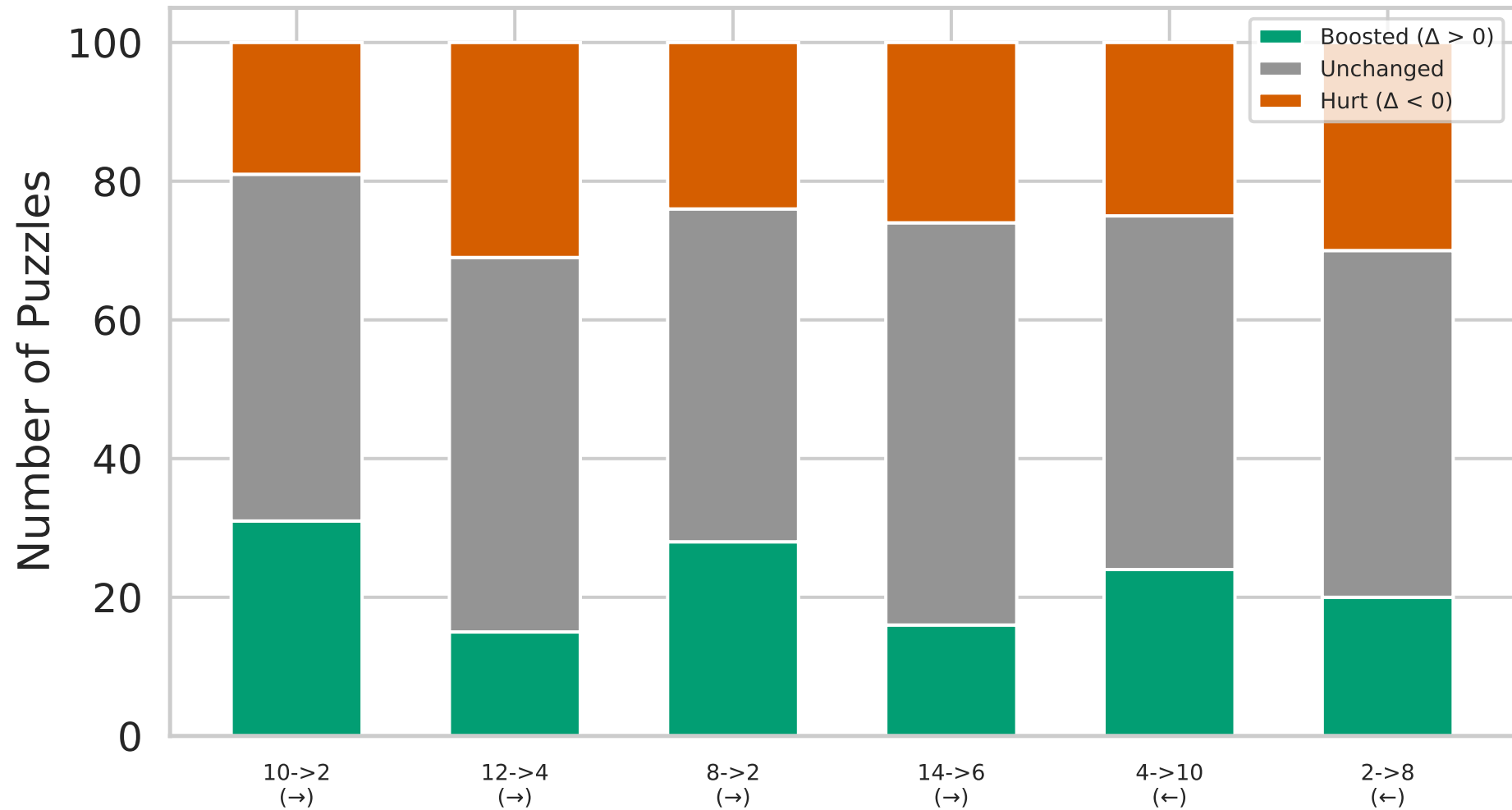
Time-Shift: Per-Puzzle Outcome Distribution
